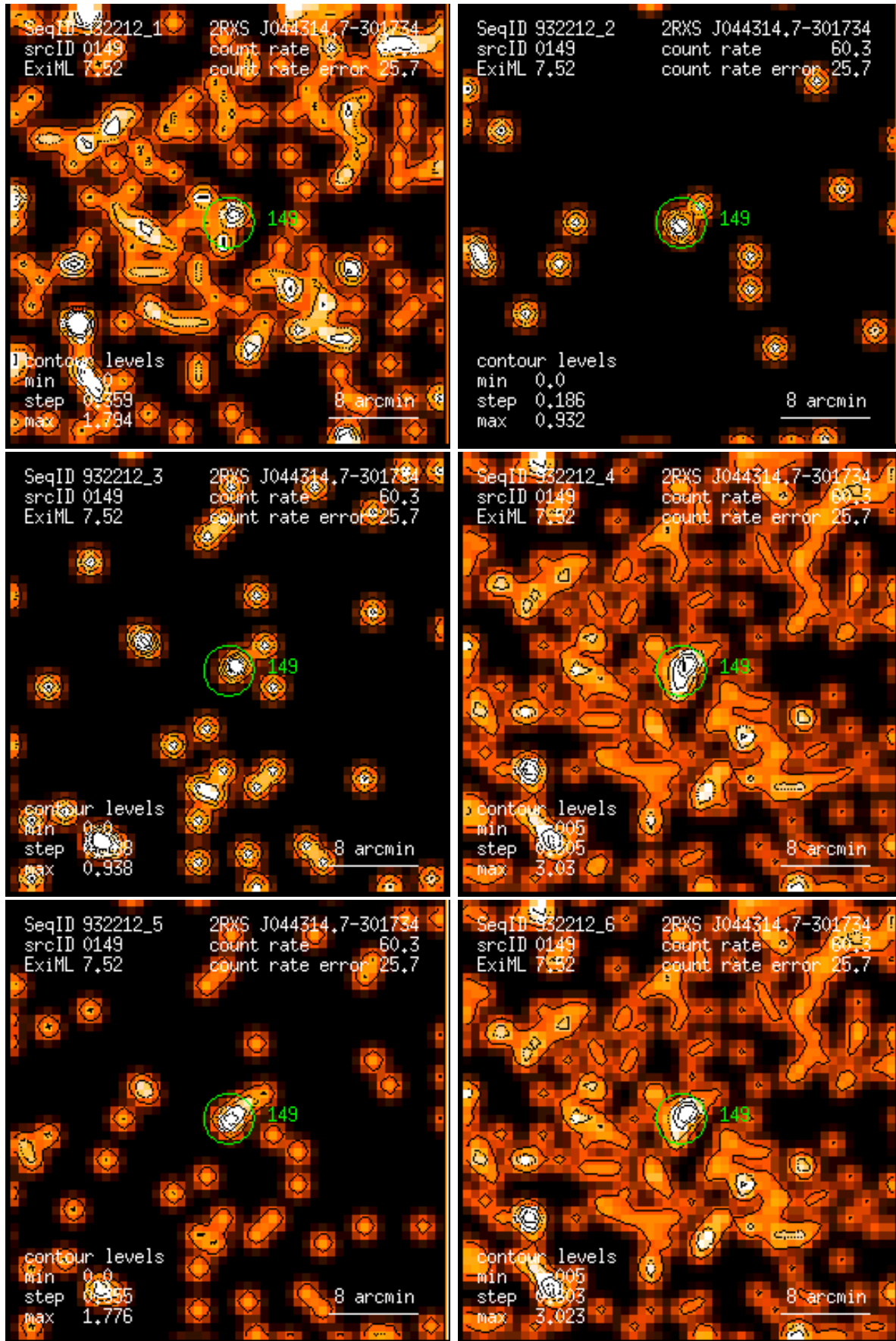
Figure 149: RASS 932212: detection 0149: band rate images, Gaussian filter: (1) PSPC channels 11 – 41, (2) 52 – 90, (3) 91 – 201, (4) 11 – 235, (5) 52 – 201, (6) 11 – 201. Broad band rates in counts/ks. Band rate contour levels in counts/ks/arcmin 2 .
