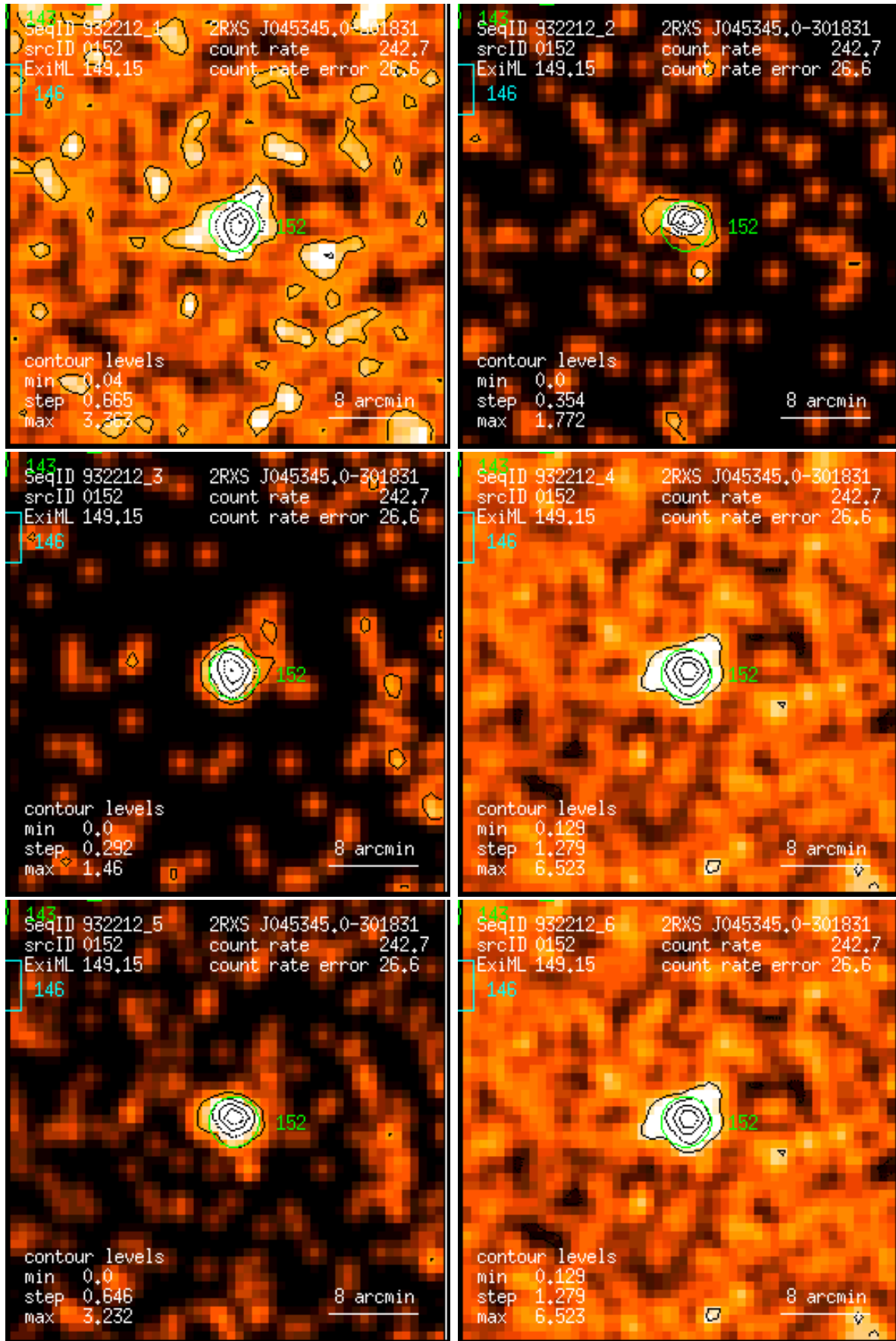
Figure 152: RASS 932212: detection 0152: band rate images, Gaussian filter: (1) PSPC channels 11 – 41, (2) 52 – 90, (3) 91 – 201, (4) 11 – 235, (5) 52 – 201, (6) 11 – 201. Broad band rates in counts/ks. Band rate contour levels in counts/ks/arcmin 2 .
