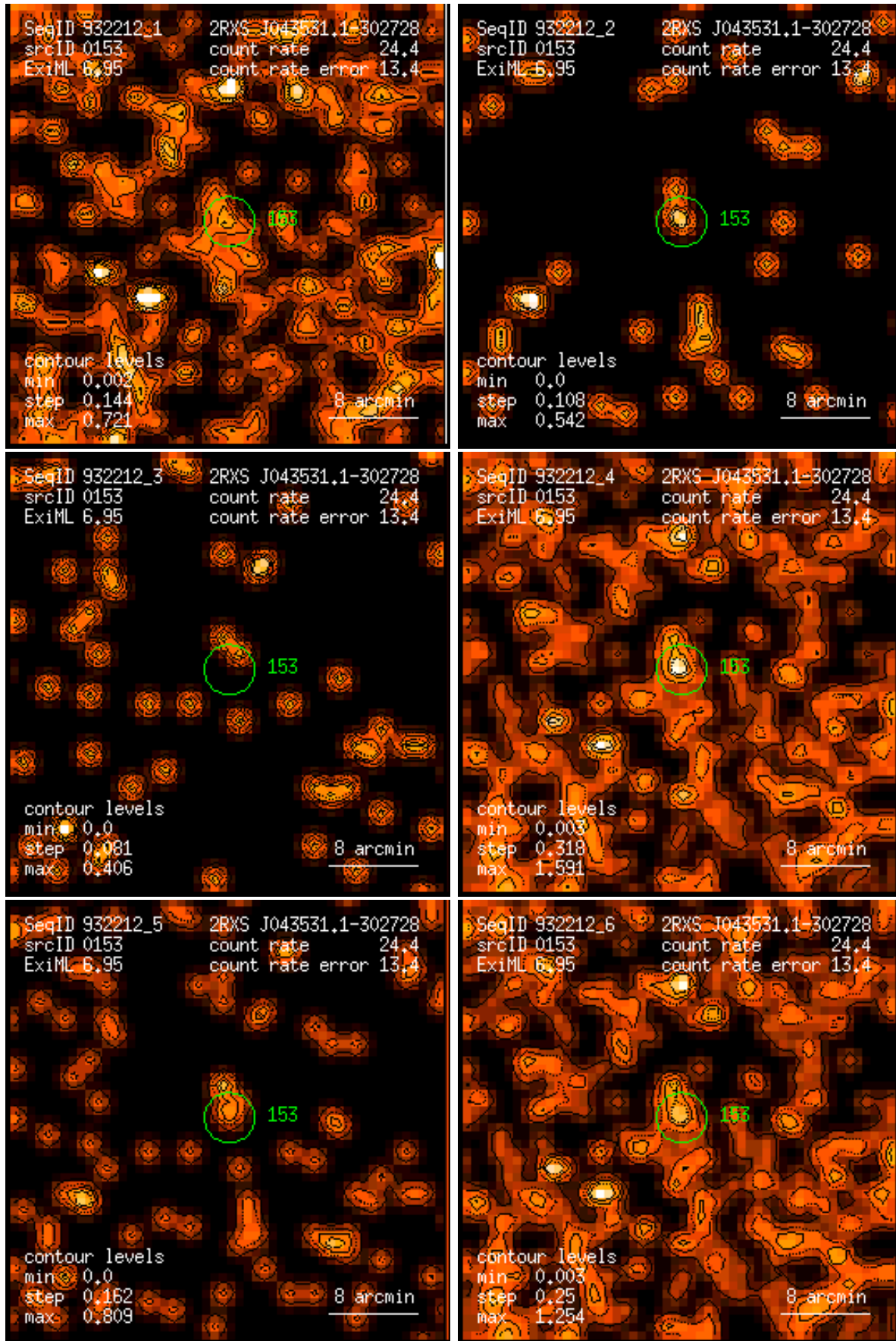
Figure 153: RASS 932212: detection 0153: band rate images, Gaussian filter: (1) PSPC channels 11 – 41, (2) 52 – 90, (3) 91 – 201, (4) 11 – 235, (5) 52 – 201, (6) 11 – 201. Broad band rates in counts/ks. Band rate contour levels in counts/ks/arcmin 2 .
