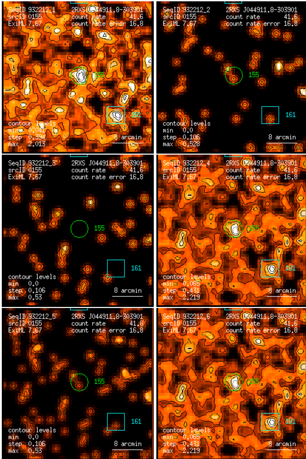
Figure 155: RASS 932212: detection 0155: band rate images, Gaussian filter: (1) PSPC channels 11 – 41, (2) 52 – 90, (3) 91 – 201, (4) 11 – 235, (5) 52 – 201, (6) 11 – 201. Broad band rates in counts/ks. Band rate contour levels in counts/ks/arcmin 2 .
