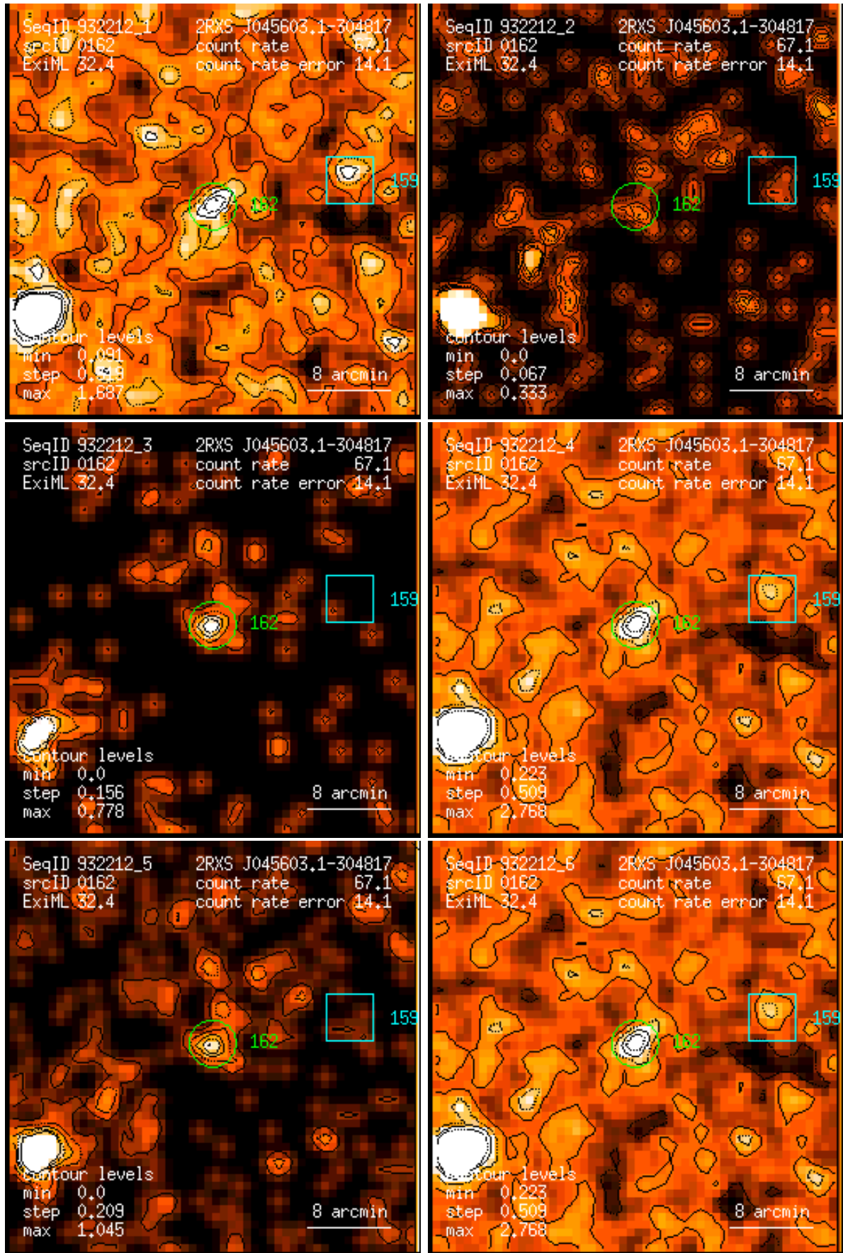
Figure 162: RASS 932212: detection 0162: band rate images, Gaussian filter: (1) PSPC channels 11 – 41, (2) 52 – 90, (3) 91 – 201, (4) 11 – 235, (5) 52 – 201, (6) 11 – 201. Broad band rates in counts/ks. Band rate contour levels in counts/ks/arcmin 2 .
