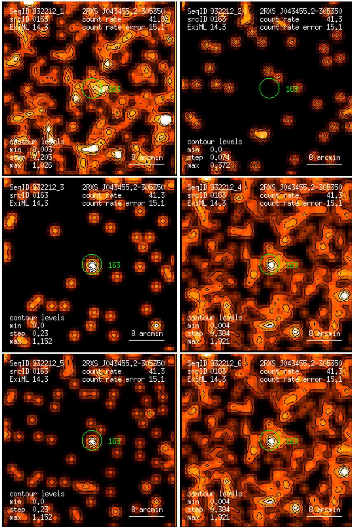
Figure 163: RASS 932212: detection 0163: band rate images, Gaussian filter: (1) PSPC channels 11 – 41, (2) 52 – 90, (3) 91 – 201, (4) 11 – 235, (5) 52 – 201, (6) 11 – 201. Broad band rates in counts/ks. Band rate contour levels in counts/ks/arcmin 2 .
