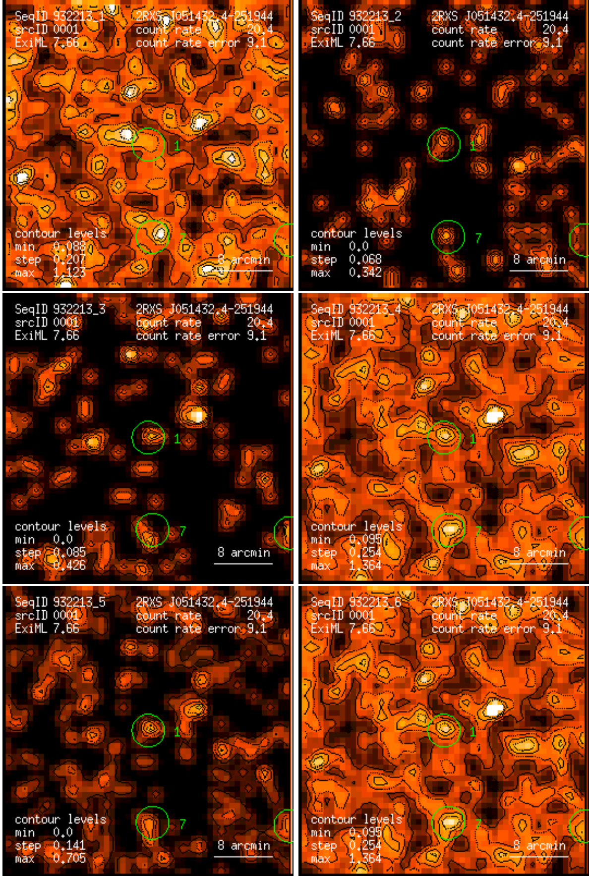
Figure 1: RASS 932213: detection 0001: band rate images, Gaussian filter: (1) PSPC channels 11 – 41, (2) 52 – 90, (3) 91 – 201, (4) 11 – 235, (5) 52 – 201, (6) 11 – 201. Broad band rates in counts/ks. Band rate contour levels in counts/ks/arcmin 2 .
