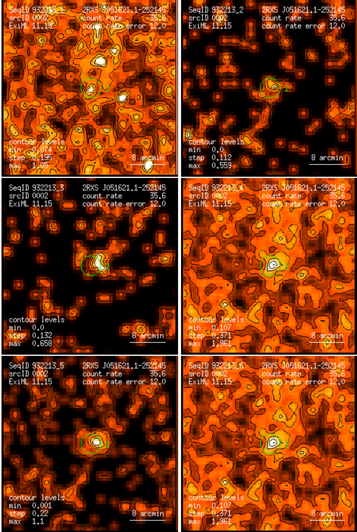
Figure 2: RASS 932213: detection 0002: band rate images, Gaussian filter: (1) PSPC channels 11 – 41, (2) 52 – 90, (3) 91 – 201, (4) 11 – 235, (5) 52 – 201, (6) 11 – 201. Broad band rates in counts/ks. Band rate contour levels in counts/ks/arcmin 2 .
