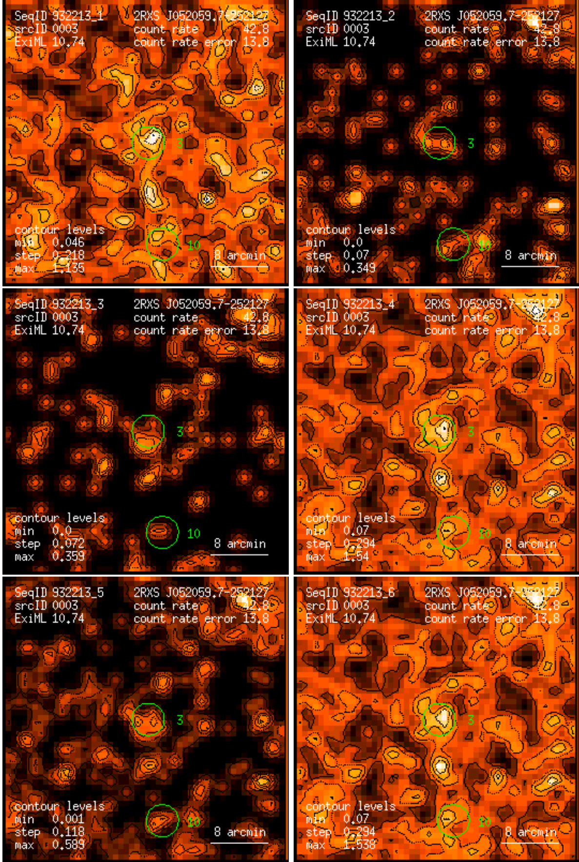
Figure 3: RASS 932213: detection 0003: band rate images, Gaussian filter: (1) PSPC channels 11 – 41, (2) 52 – 90, (3) 91 – 201, (4) 11 – 235, (5) 52 – 201, (6) 11 – 201. Broad band rates in counts/ks. Band rate contour levels in counts/ks/arcmin 2 .
