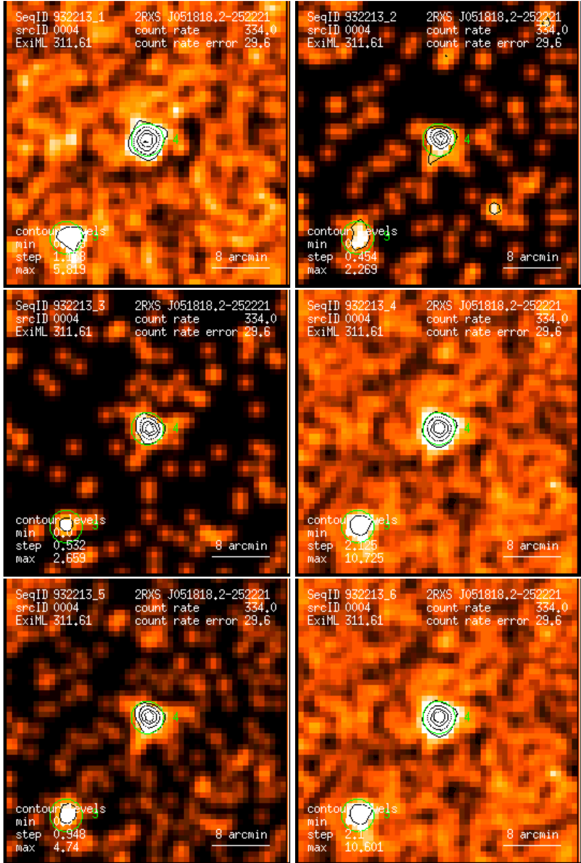
Figure 4: RASS 932213: detection 0004: band rate images, Gaussian filter: (1) PSPC channels 11 – 41, (2) 52 – 90, (3) 91 – 201, (4) 11 – 235, (5) 52 – 201, (6) 11 – 201. Broad band rates in counts/ks. Band rate contour levels in counts/ks/arcmin 2 .
