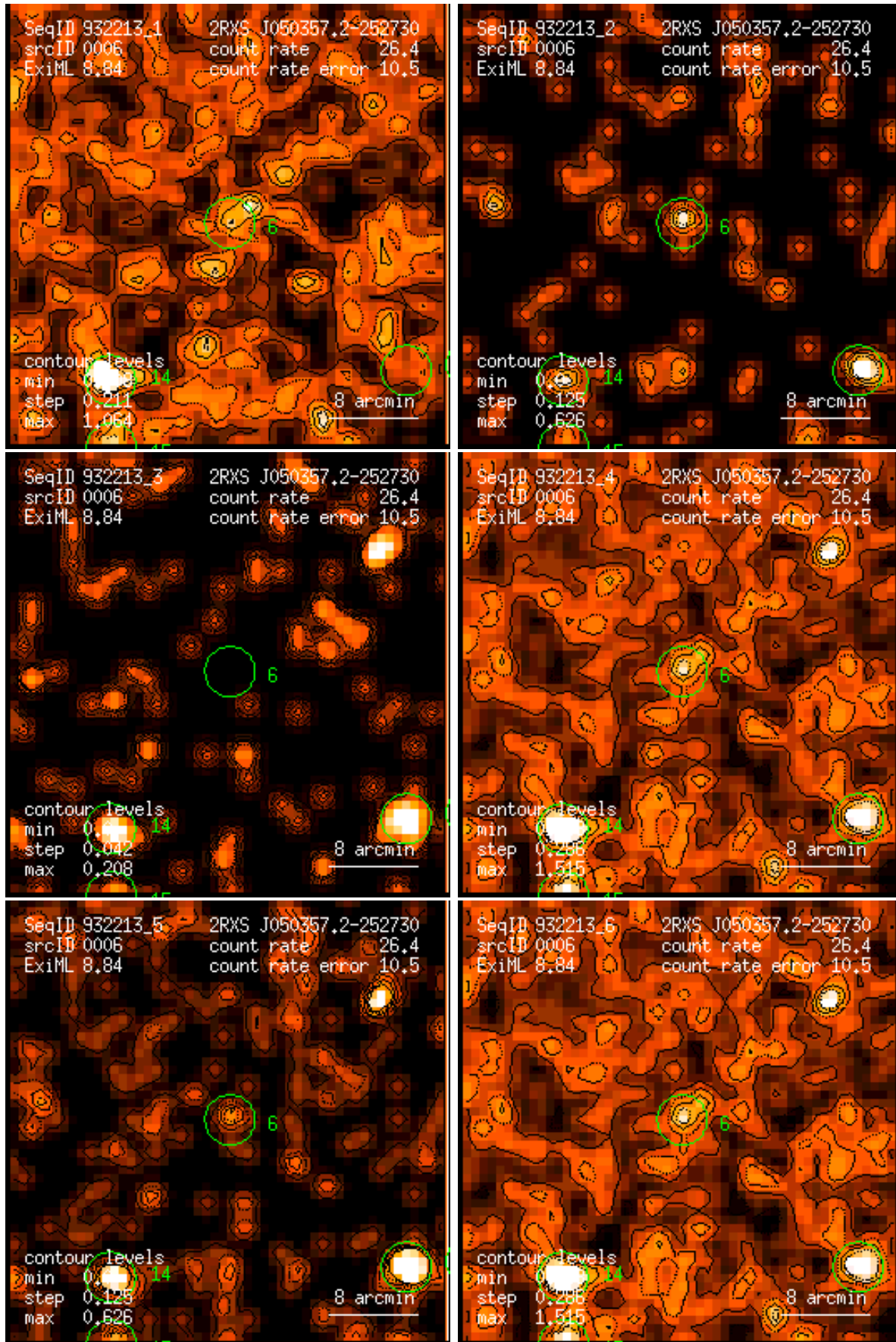
Figure 6: RASS 932213: detection 0006: band rate images, Gaussian filter: (1) PSPC channels 11 – 41, (2) 52 – 90, (3) 91 – 201, (4) 11 – 235, (5) 52 – 201, (6) 11 – 201. Broad band rates in counts/ks. Band rate contour levels in counts/ks/arcmin 2 .
