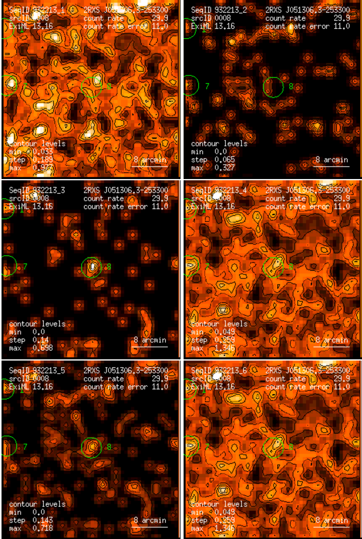
Figure 8: RASS 932213: detection 0008: band rate images, Gaussian filter: (1) PSPC channels 11 – 41, (2) 52 – 90, (3) 91 – 201, (4) 11 – 235, (5) 52 – 201, (6) 11 – 201. Broad band rates in counts/ks. Band rate contour levels in counts/ks/arcmin 2 .
