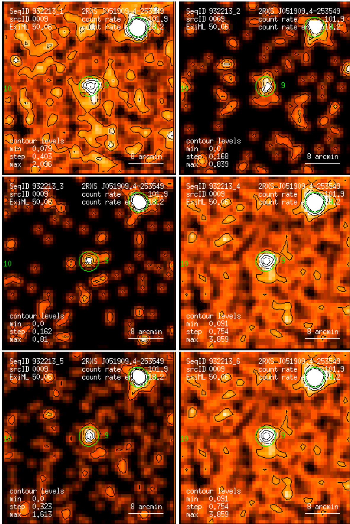
Figure 9: RASS 932213: detection 0009: band rate images, Gaussian filter: (1) PSPC channels 11 – 41, (2) 52 – 90, (3) 91 – 201, (4) 11 – 235, (5) 52 – 201, (6) 11 – 201. Broad band rates in counts/ks. Band rate contour levels in counts/ks/arcmin 2 .
