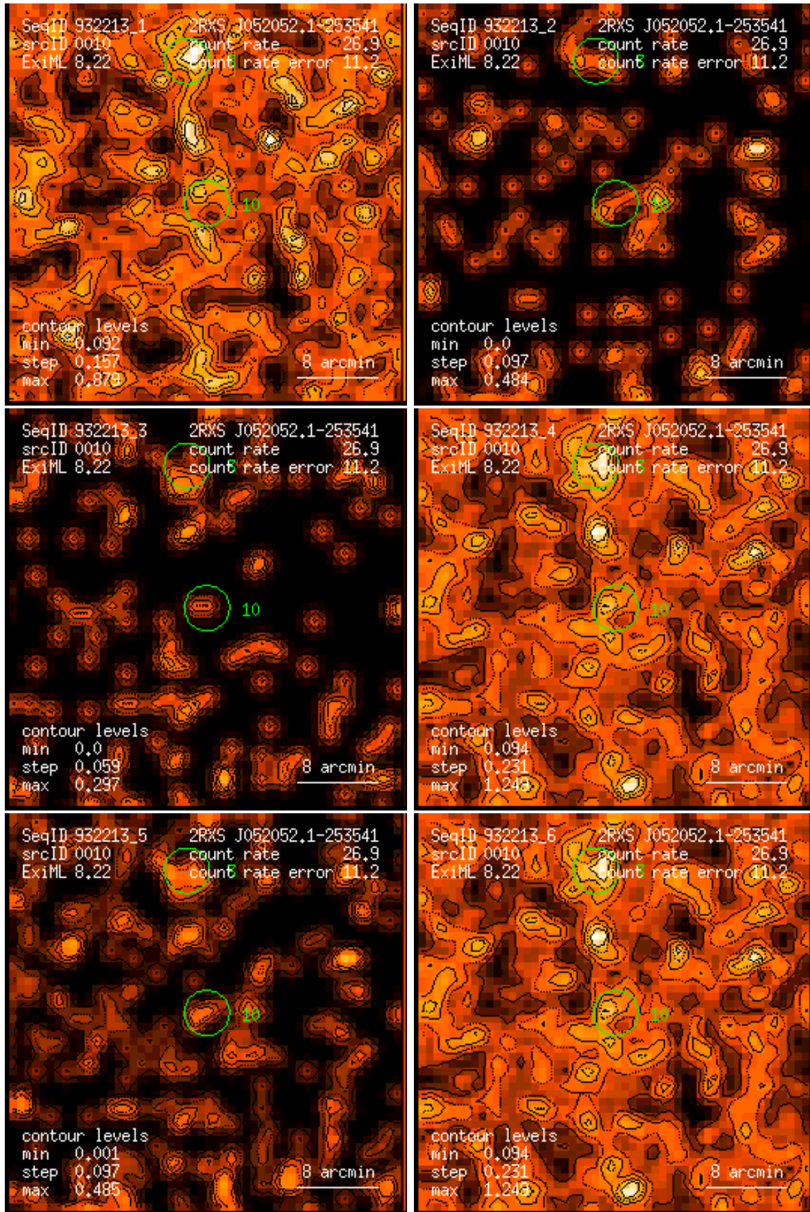
Figure 10: RASS 932213: detection 0010: band rate images, Gaussian filter: (1) PSPC channels 11 – 41, (2) 52 – 90, (3) 91 – 201, (4) 11 – 235, (5) 52 – 201, (6) 11 – 201. Broad band rates in counts/ks. Band rate contour levels in counts/ks/arcmin 2 .
