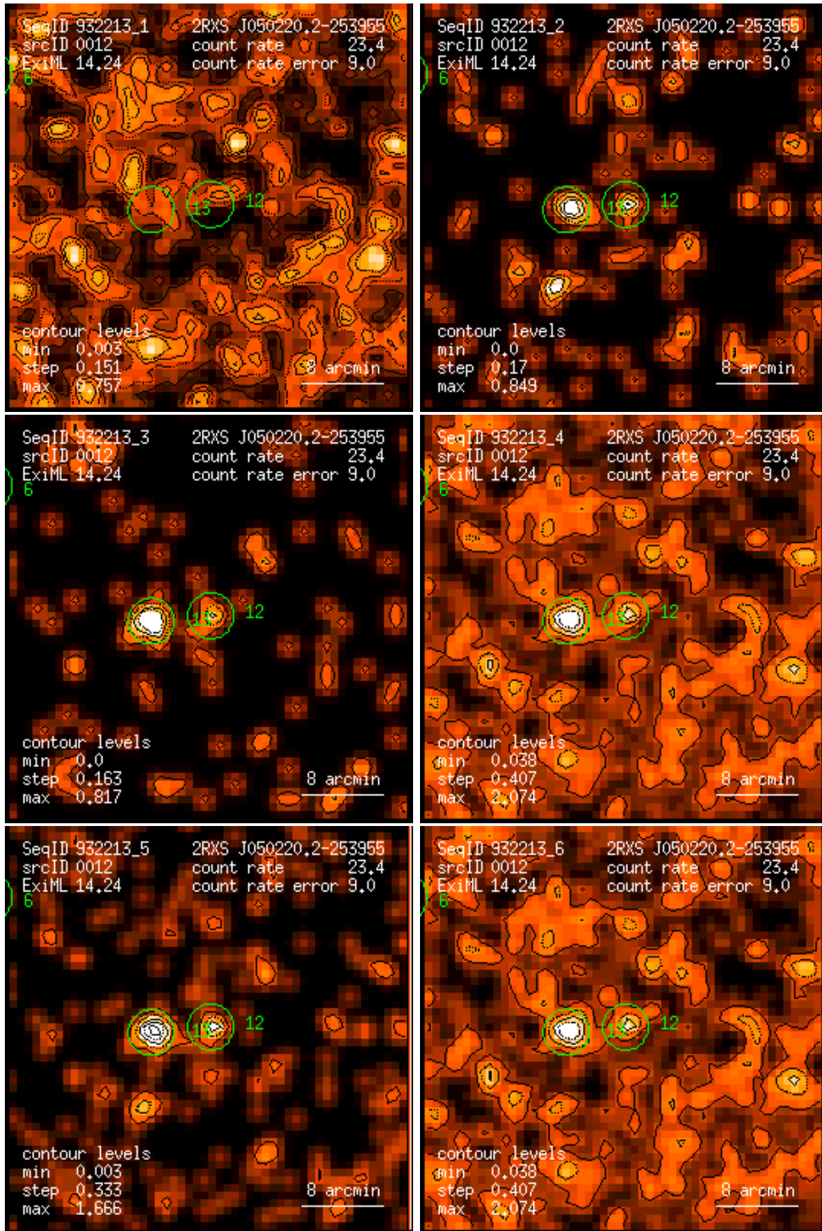
Figure 12: RASS 932213: detection 0012: band rate images, Gaussian filter: (1) PSPC channels 11 – 41, (2) 52 – 90, (3) 91 – 201, (4) 11 – 235, (5) 52 – 201, (6) 11 – 201. Broad band rates in counts/ks. Band rate contour levels in counts/ks/arcmin 2 .
