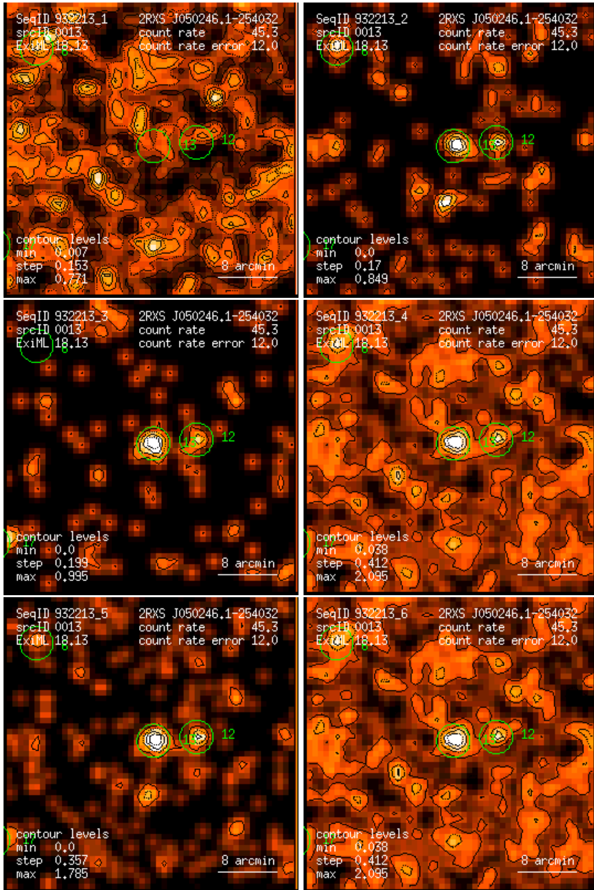
Figure 13: RASS 932213: detection 0013: band rate images, Gaussian filter: (1) PSPC channels 11 – 41, (2) 52 – 90, (3) 91 – 201, (4) 11 – 235, (5) 52 – 201, (6) 11 – 201. Broad band rates in counts/ks. Band rate contour levels in counts/ks/arcmin 2 .
