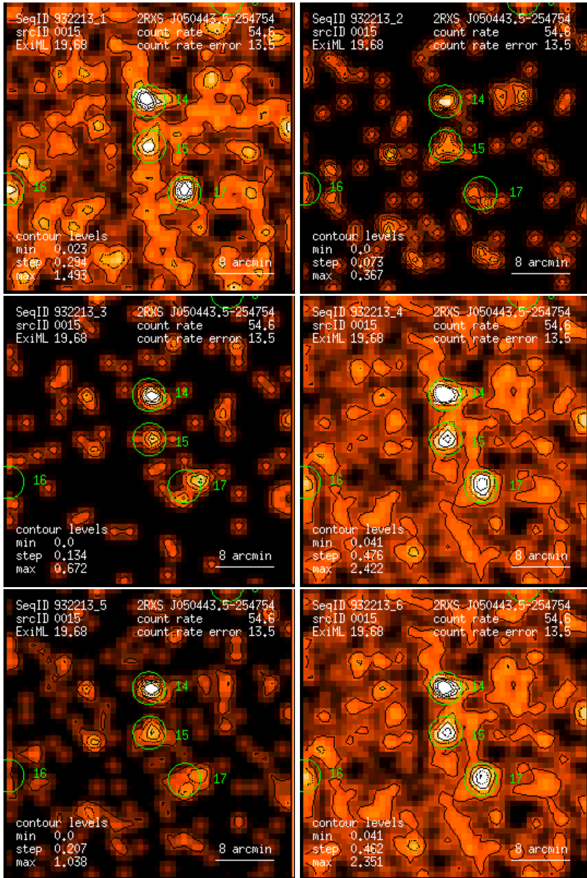
Figure 15: RASS 932213: detection 0015: band rate images, Gaussian filter: (1) PSPC channels 11 – 41, (2) 52 – 90, (3) 91 – 201, (4) 11 – 235, (5) 52 – 201, (6) 11 – 201. Broad band rates in counts/ks. Band rate contour levels in counts/ks/arcmin 2 .
