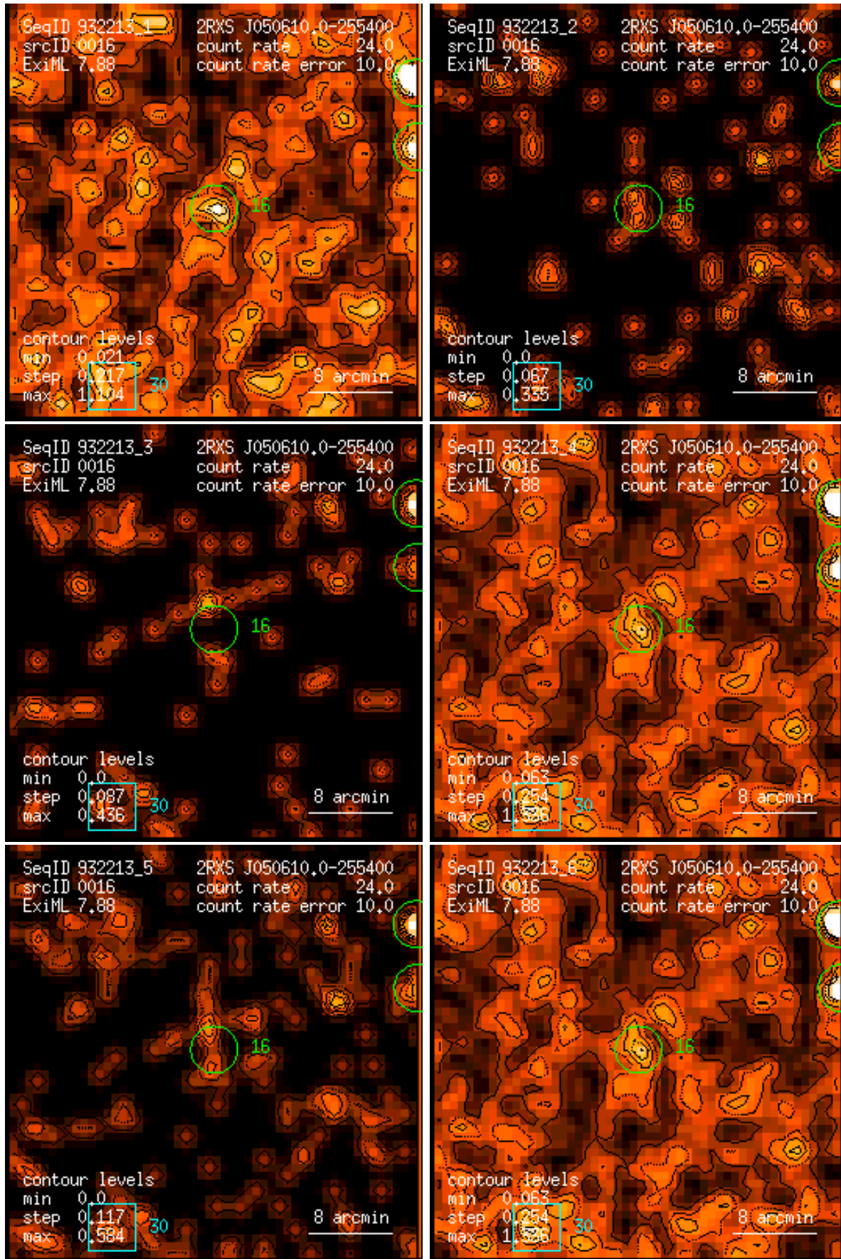
Figure 16: RASS 932213: detection 0016: band rate images, Gaussian filter: (1) PSPC channels 11 – 41, (2) 52 – 90, (3) 91 – 201, (4) 11 – 235, (5) 52 – 201, (6) 11 – 201. Broad band rates in counts/ks. Band rate contour levels in counts/ks/arcmin 2 .
