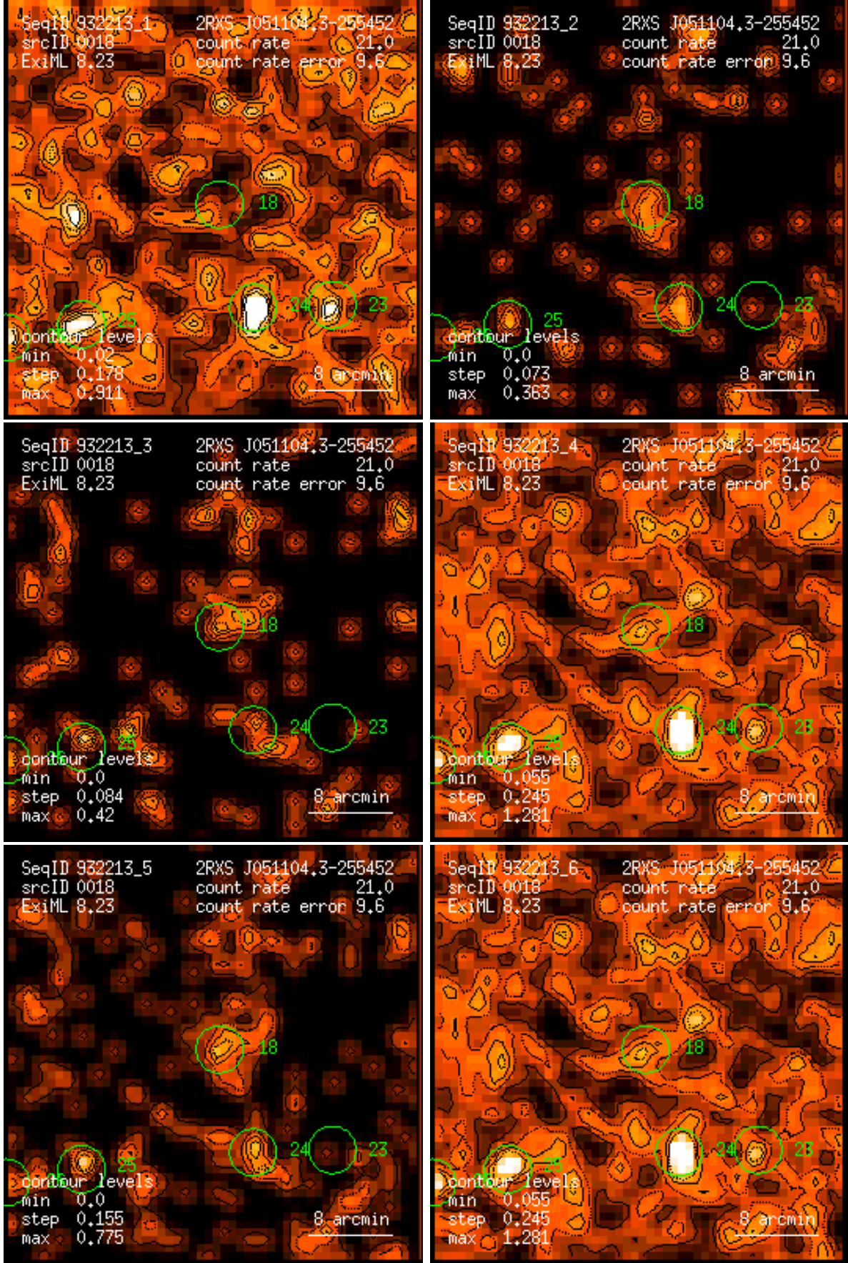
Figure 18: RASS 932213: detection 0018: band rate images, Gaussian filter: (1) PSPC channels 11 – 41, (2) 52 – 90, (3) 91 – 201, (4) 11 – 235, (5) 52 – 201, (6) 11 – 201. Broad band rates in counts/ks. Band rate contour levels in counts/ks/arcmin 2 .
