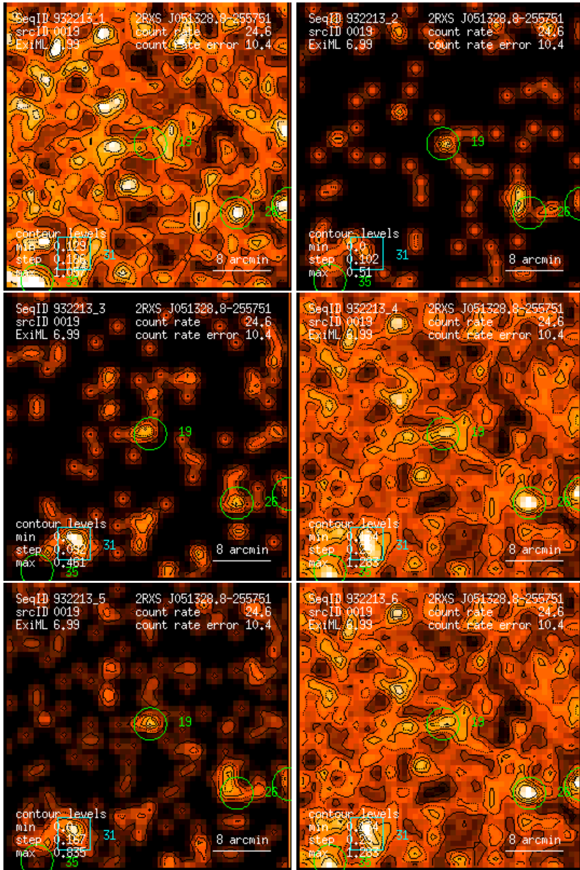
Figure 19: RASS 932213: detection 0019: band rate images, Gaussian filter: (1) PSPC channels 11 – 41, (2) 52 – 90, (3) 91 – 201, (4) 11 – 235, (5) 52 – 201, (6) 11 – 201. Broad band rates in counts/ks. Band rate contour levels in counts/ks/arcmin 2 .
