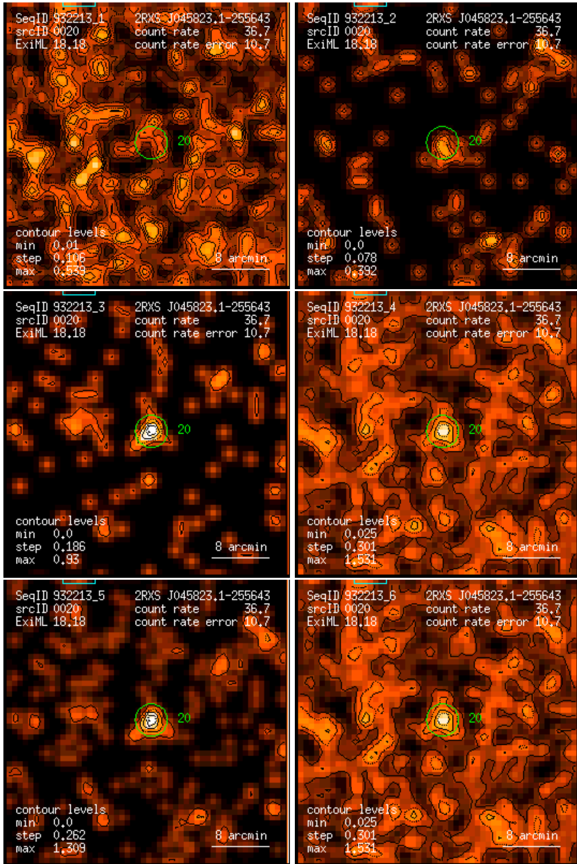
Figure 20: RASS 932213: detection 0020: band rate images, Gaussian filter: (1) PSPC channels 11 – 41, (2) 52 – 90, (3) 91 – 201, (4) 11 – 235, (5) 52 – 201, (6) 11 – 201. Broad band rates in counts/ks. Band rate contour levels in counts/ks/arcmin 2 .
