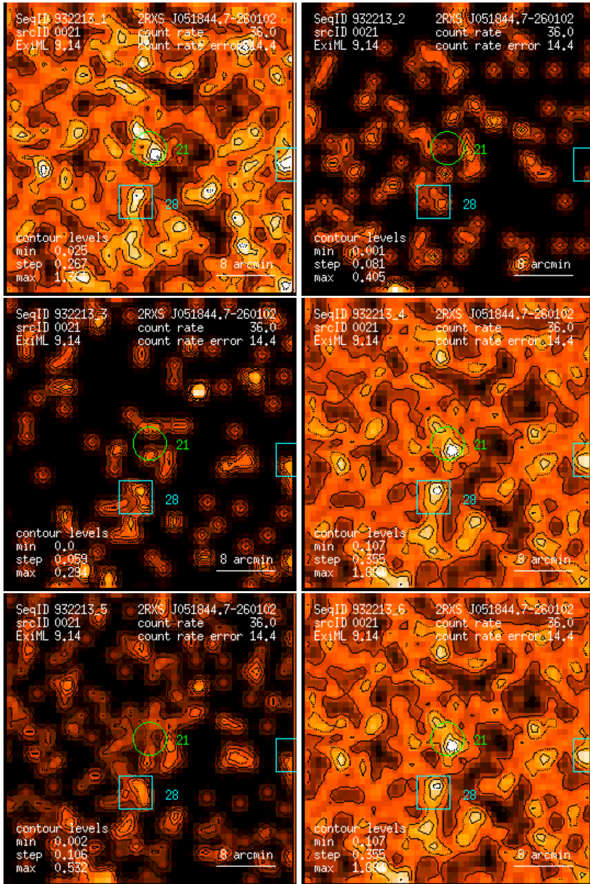
Figure 21: RASS 932213: detection 0021: band rate images, Gaussian filter: (1) PSPC channels 11 – 41, (2) 52 – 90, (3) 91 – 201, (4) 11 – 235, (5) 52 – 201, (6) 11 – 201. Broad band rates in counts/ks. Band rate contour levels in counts/ks/arcmin 2 .
