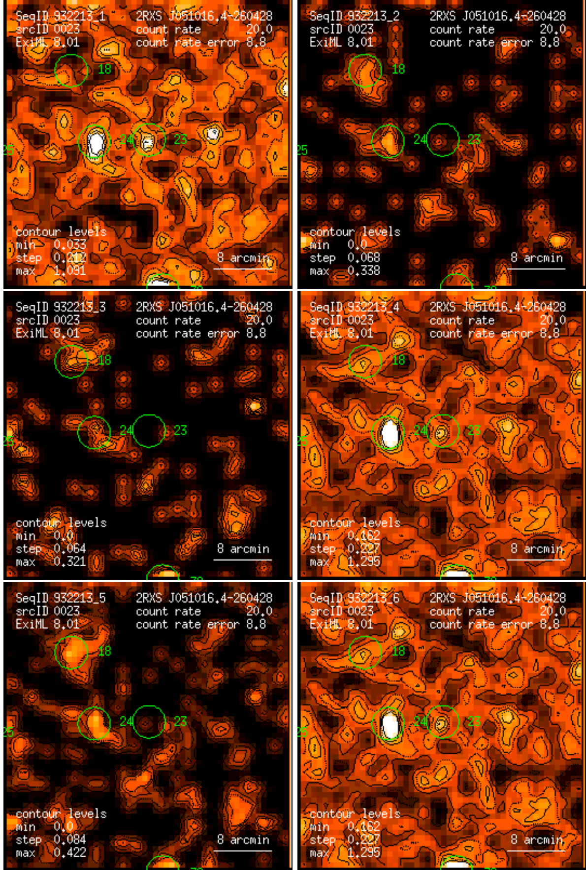
Figure 23: RASS 932213: detection 0023: band rate images, Gaussian filter: (1) PSPC channels 11 – 41, (2) 52 – 90, (3) 91 – 201, (4) 11 – 235, (5) 52 – 201, (6) 11 – 201. Broad band rates in counts/ks. Band rate contour levels in counts/ks/arcmin 2 .
