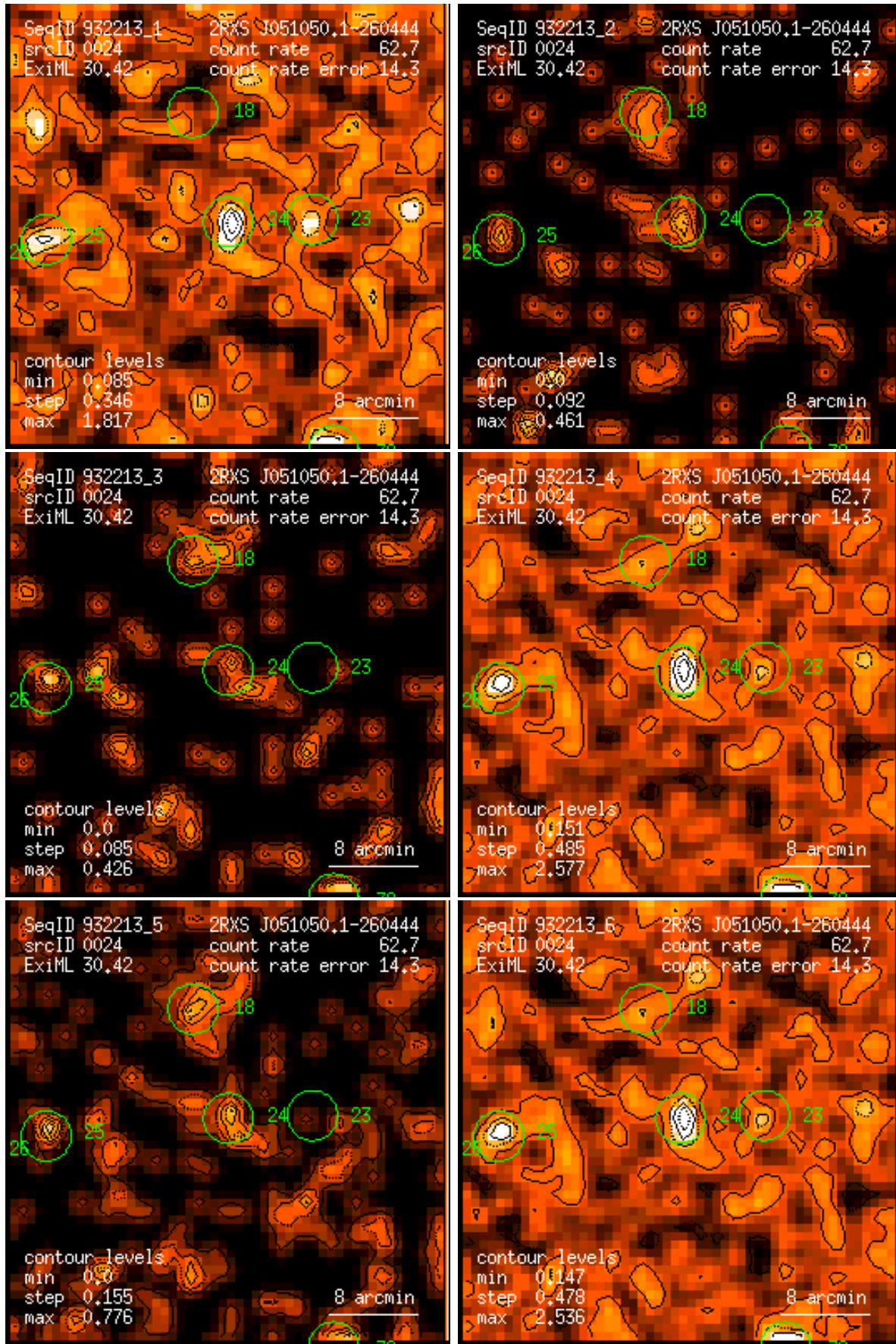
Figure 24: RASS 932213: detection 0024: band rate images, Gaussian filter: (1) PSPC channels 11 – 41, (2) 52 – 90, (3) 91 – 201, (4) 11 – 235, (5) 52 – 201, (6) 11 – 201. Broad band rates in counts/ks. Band rate contour levels in counts/ks/arcmin 2 .
