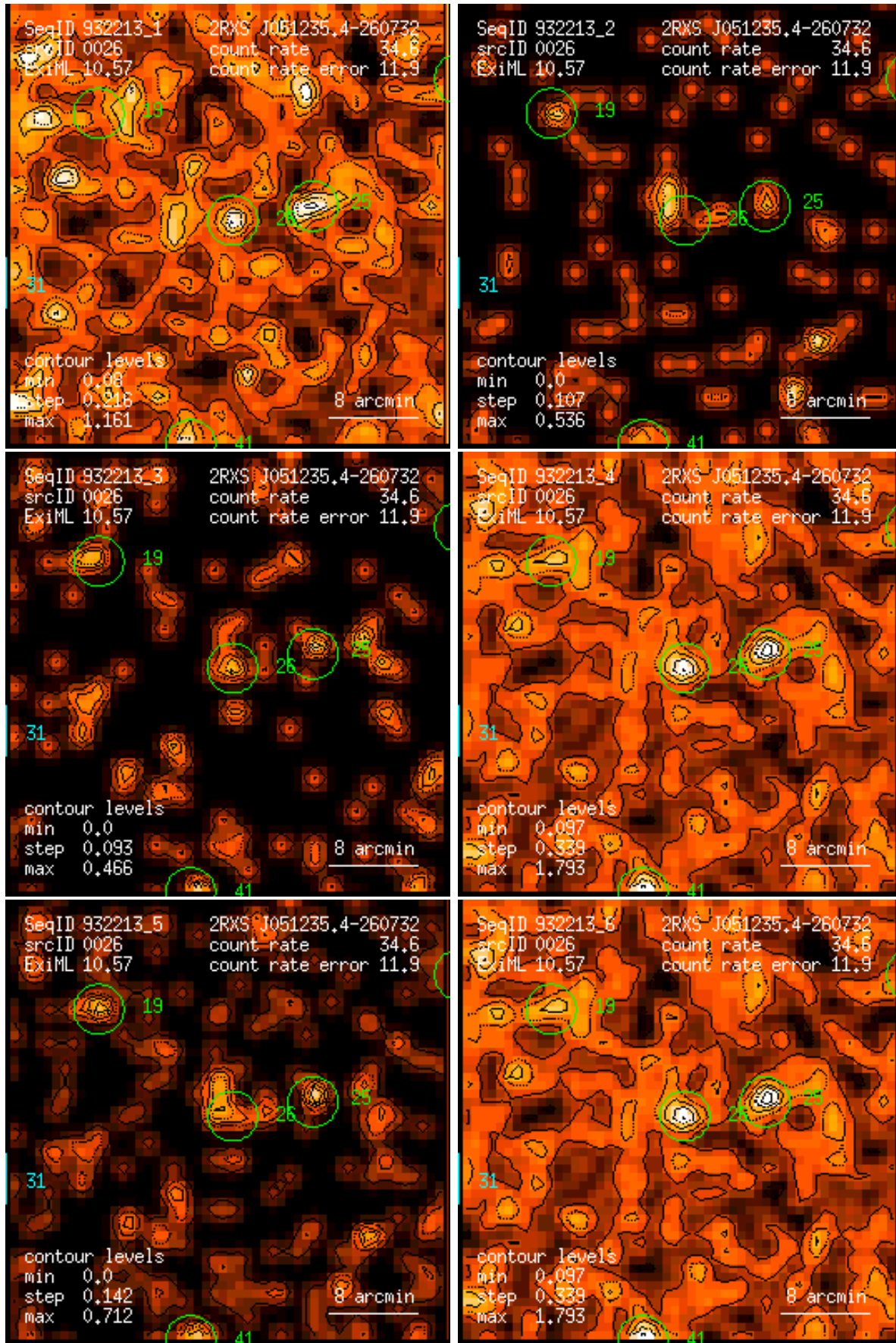
Figure 26: RASS 932213: detection 0026: band rate images, Gaussian filter: (1) PSPC channels 11 – 41, (2) 52 – 90, (3) 91 – 201, (4) 11 – 235, (5) 52 – 201, (6) 11 – 201. Broad band rates in counts/ks. Band rate contour levels in counts/ks/arcmin 2 .
