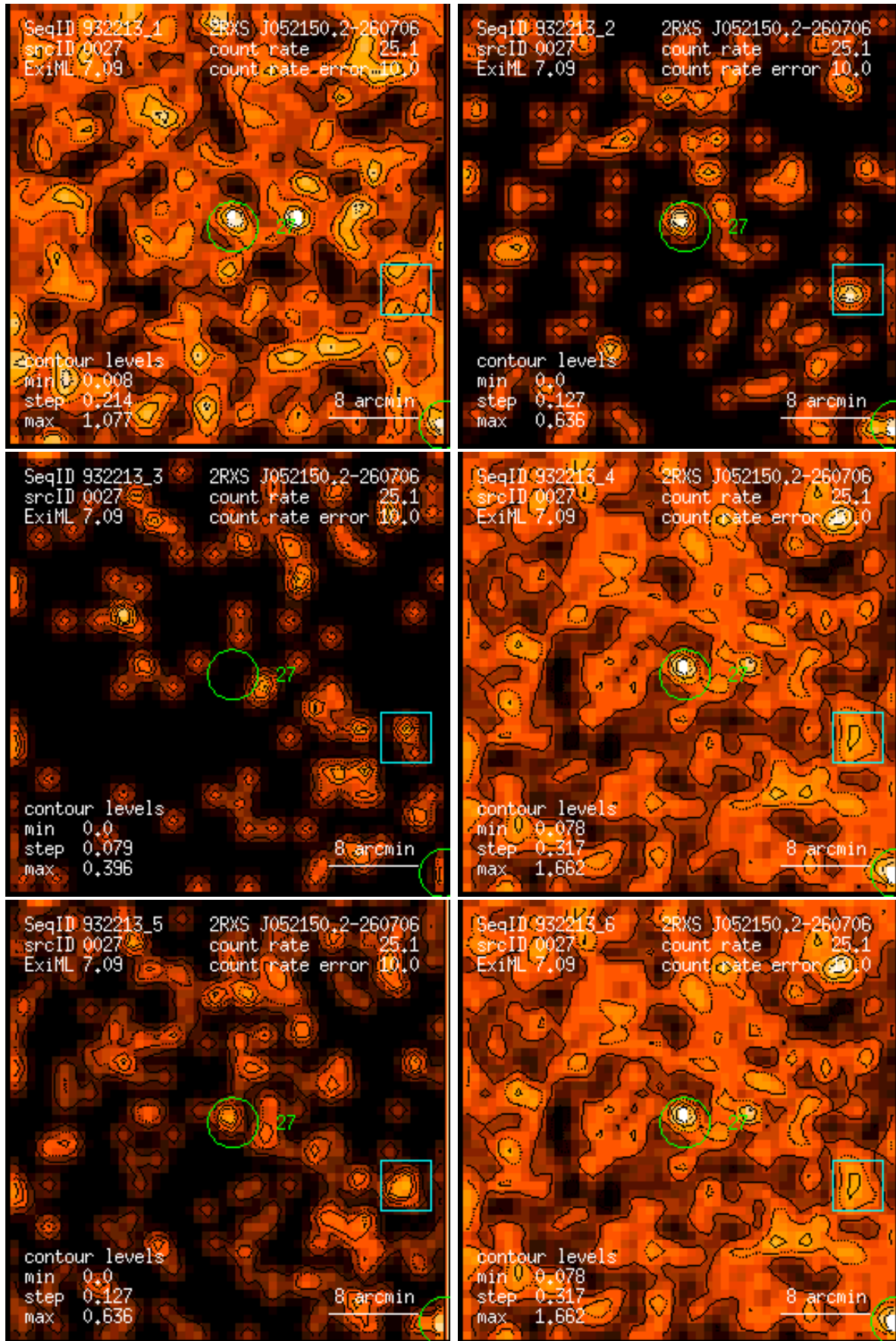
Figure 27: RASS 932213: detection 0027: band rate images, Gaussian filter: (1) PSPC channels 11 – 41, (2) 52 – 90, (3) 91 – 201, (4) 11 – 235, (5) 52 – 201, (6) 11 – 201. Broad band rates in counts/ks. Band rate contour levels in counts/ks/arcmin 2 .
