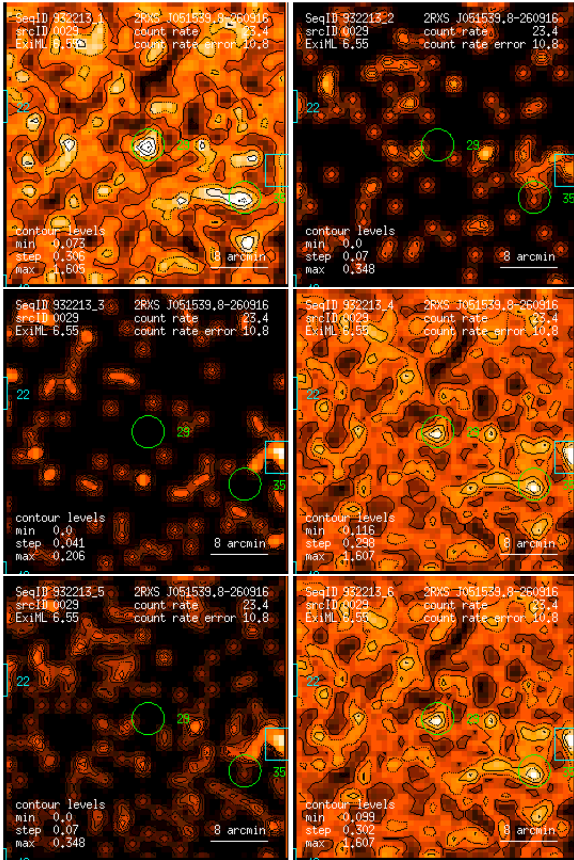
Figure 29: RASS 932213: detection 0029: band rate images, Gaussian filter: (1) PSPC channels 11 – 41, (2) 52 – 90, (3) 91 – 201, (4) 11 – 235, (5) 52 – 201, (6) 11 – 201. Broad band rates in counts/ks. Band rate contour levels in counts/ks/arcmin 2 .
