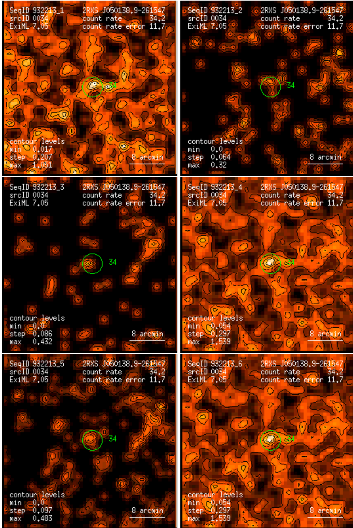
Figure 34: RASS 932213: detection 0034: band rate images, Gaussian filter: (1) PSPC channels 11 – 41, (2) 52 – 90, (3) 91 – 201, (4) 11 – 235, (5) 52 – 201, (6) 11 – 201. Broad band rates in counts/ks. Band rate contour levels in counts/ks/arcmin 2 .
