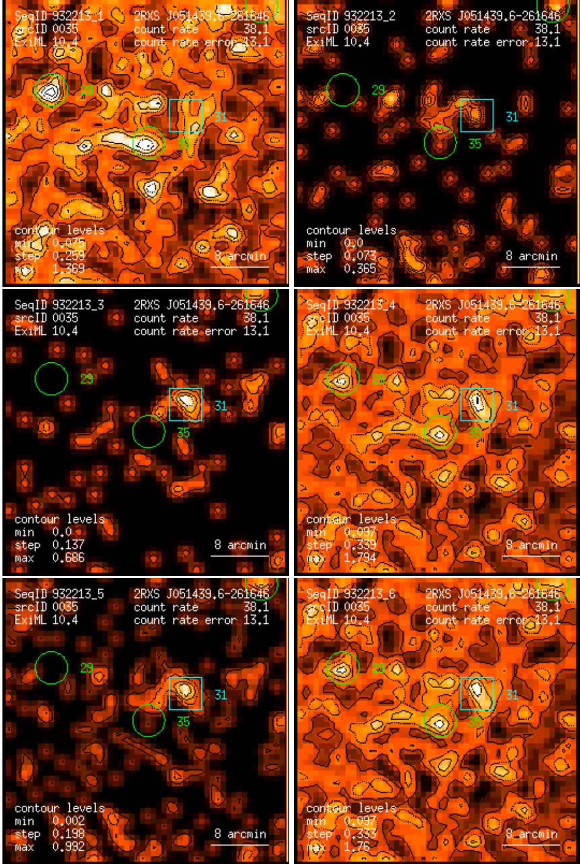
Figure 35: RASS 932213: detection 0035: band rate images, Gaussian filter: (1) PSPC channels 11 – 41, (2) 52 – 90, (3) 91 – 201, (4) 11 – 235, (5) 52 – 201, (6) 11 – 201. Broad band rates in counts/ks. Band rate contour levels in counts/ks/arcmin 2 .
