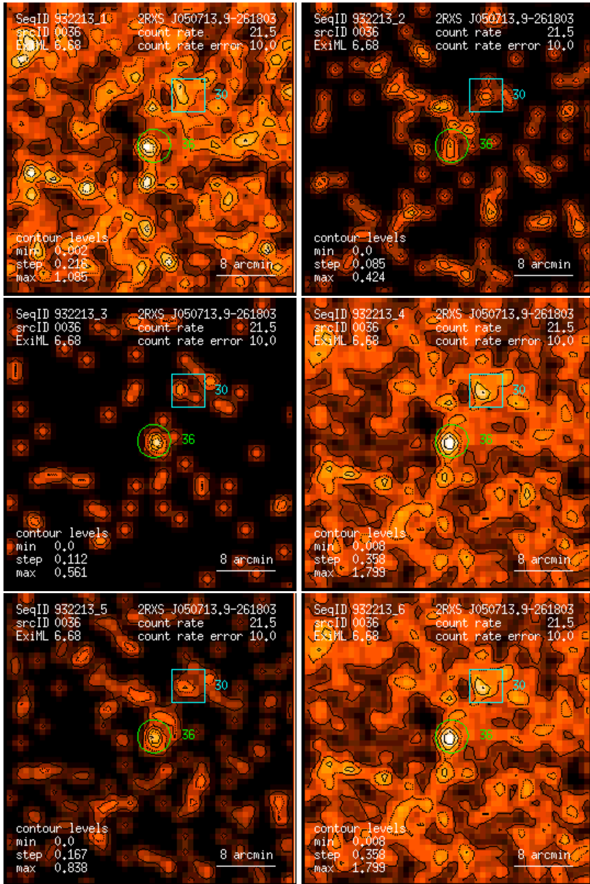
Figure 36: RASS 932213: detection 0036: band rate images, Gaussian filter: (1) PSPC channels 11 – 41, (2) 52 – 90, (3) 91 – 201, (4) 11 – 235, (5) 52 – 201, (6) 11 – 201. Broad band rates in counts/ks. Band rate contour levels in counts/ks/arcmin 2 .
