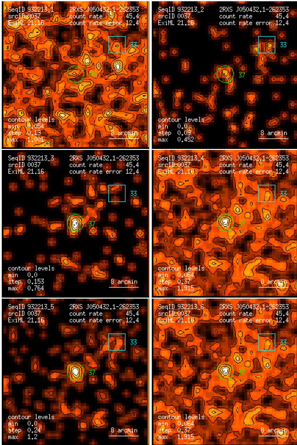
Figure 37: RASS 932213: detection 0037: band rate images, Gaussian filter: (1) PSPC channels 11 – 41, (2) 52 – 90, (3) 91 – 201, (4) 11 – 235, (5) 52 – 201, (6) 11 – 201. Broad band rates in counts/ks. Band rate contour levels in counts/ks/arcmin 2 .
