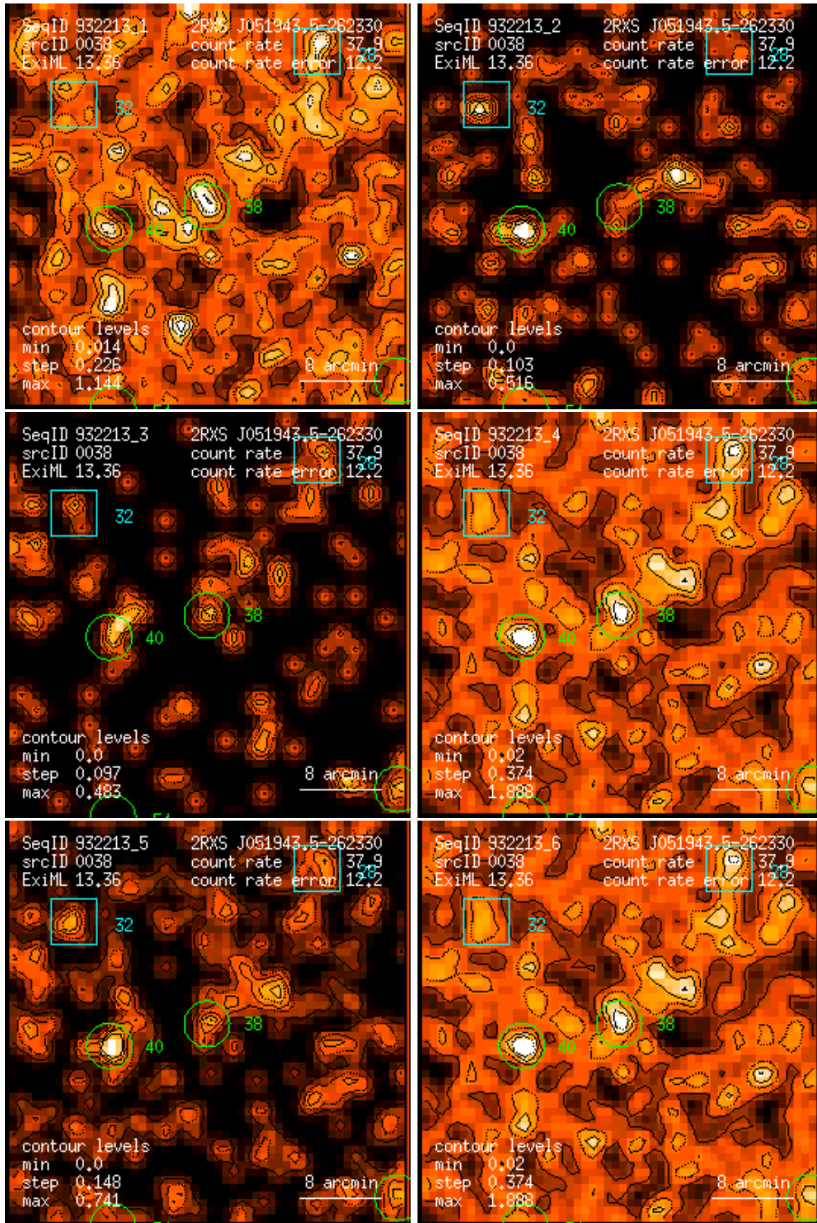
Figure 38: RASS 932213: detection 0038: band rate images, Gaussian filter: (1) PSPC channels 11 – 41, (2) 52 – 90, (3) 91 – 201, (4) 11 – 235, (5) 52 – 201, (6) 11 – 201. Broad band rates in counts/ks. Band rate contour levels in counts/ks/arcmin 2 .
