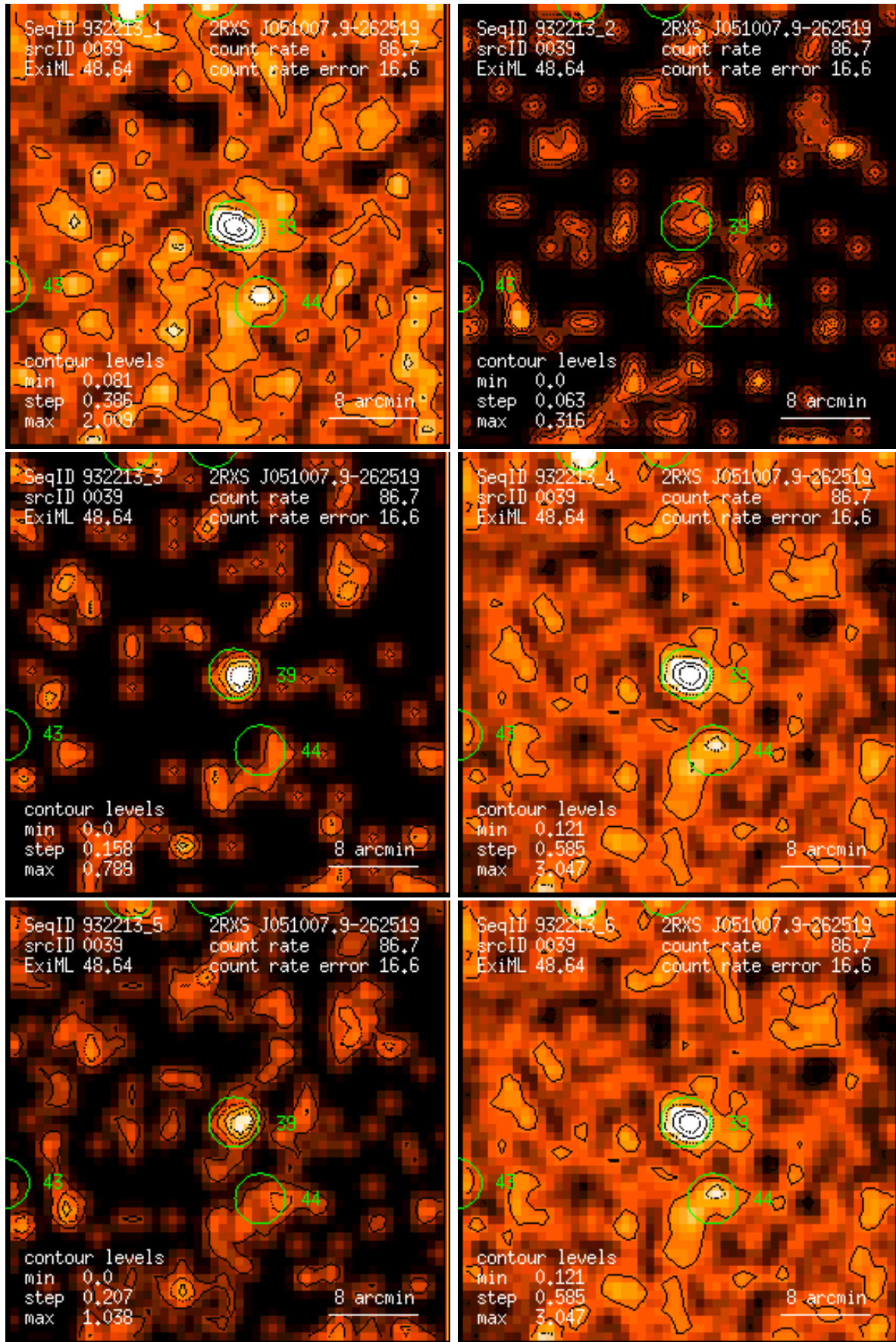
Figure 39: RASS 932213: detection 0039: band rate images, Gaussian filter: (1) PSPC channels 11 – 41, (2) 52 – 90, (3) 91 – 201, (4) 11 – 235, (5) 52 – 201, (6) 11 – 201. Broad band rates in counts/ks. Band rate contour levels in counts/ks/arcmin 2 .
