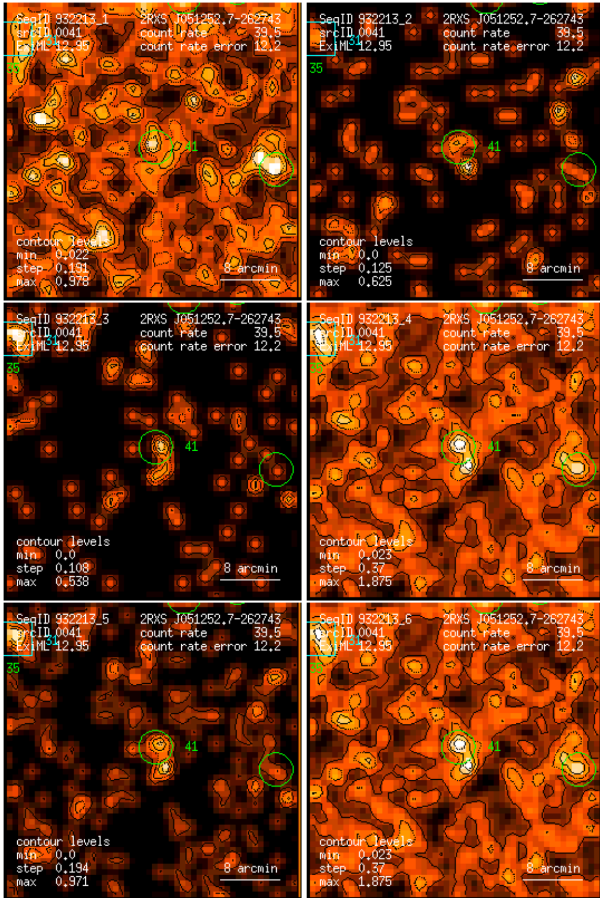
Figure 41: RASS 932213: detection 0041: band rate images, Gaussian filter: (1) PSPC channels 11 – 41, (2) 52 – 90, (3) 91 – 201, (4) 11 – 235, (5) 52 – 201, (6) 11 – 201. Broad band rates in counts/ks. Band rate contour levels in counts/ks/arcmin 2 .
