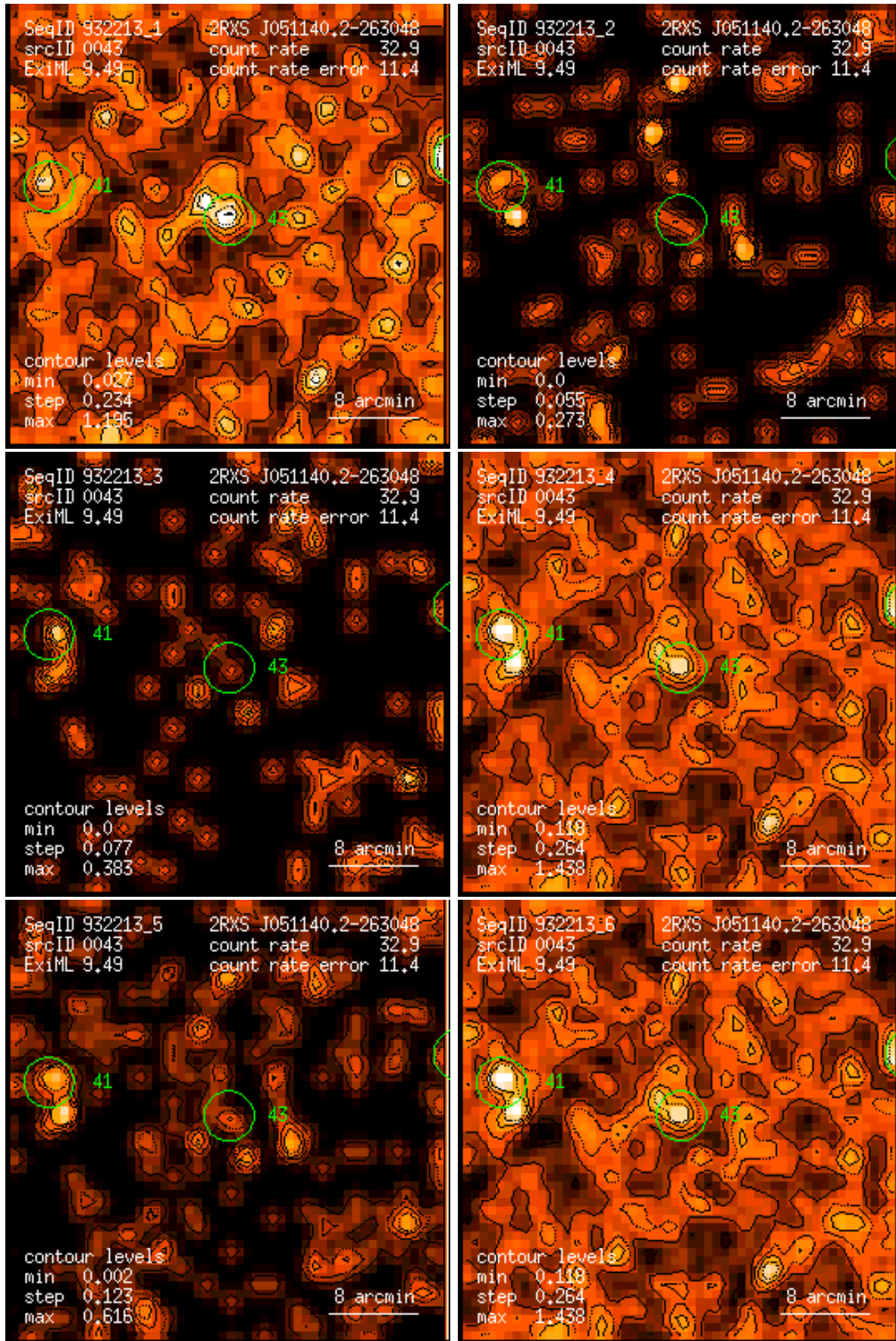
Figure 43: RASS 932213: detection 0043: band rate images, Gaussian filter: (1) PSPC channels 11 – 41, (2) 52 – 90, (3) 91 – 201, (4) 11 – 235, (5) 52 – 201, (6) 11 – 201. Broad band rates in counts/ks. Band rate contour levels in counts/ks/arcmin 2 .
