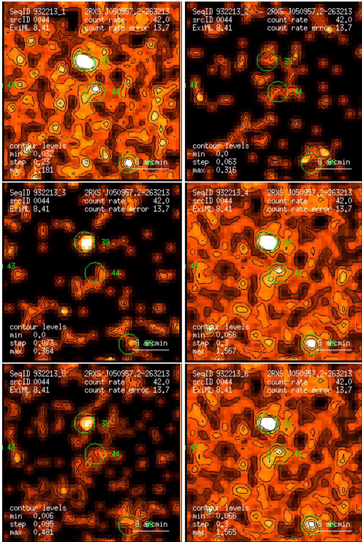
Figure 44: RASS 932213: detection 0044: band rate images, Gaussian filter: (1) PSPC channels 11 – 41, (2) 52 – 90, (3) 91 – 201, (4) 11 – 235, (5) 52 – 201, (6) 11 – 201. Broad band rates in counts/ks. Band rate contour levels in counts/ks/arcmin 2 .
