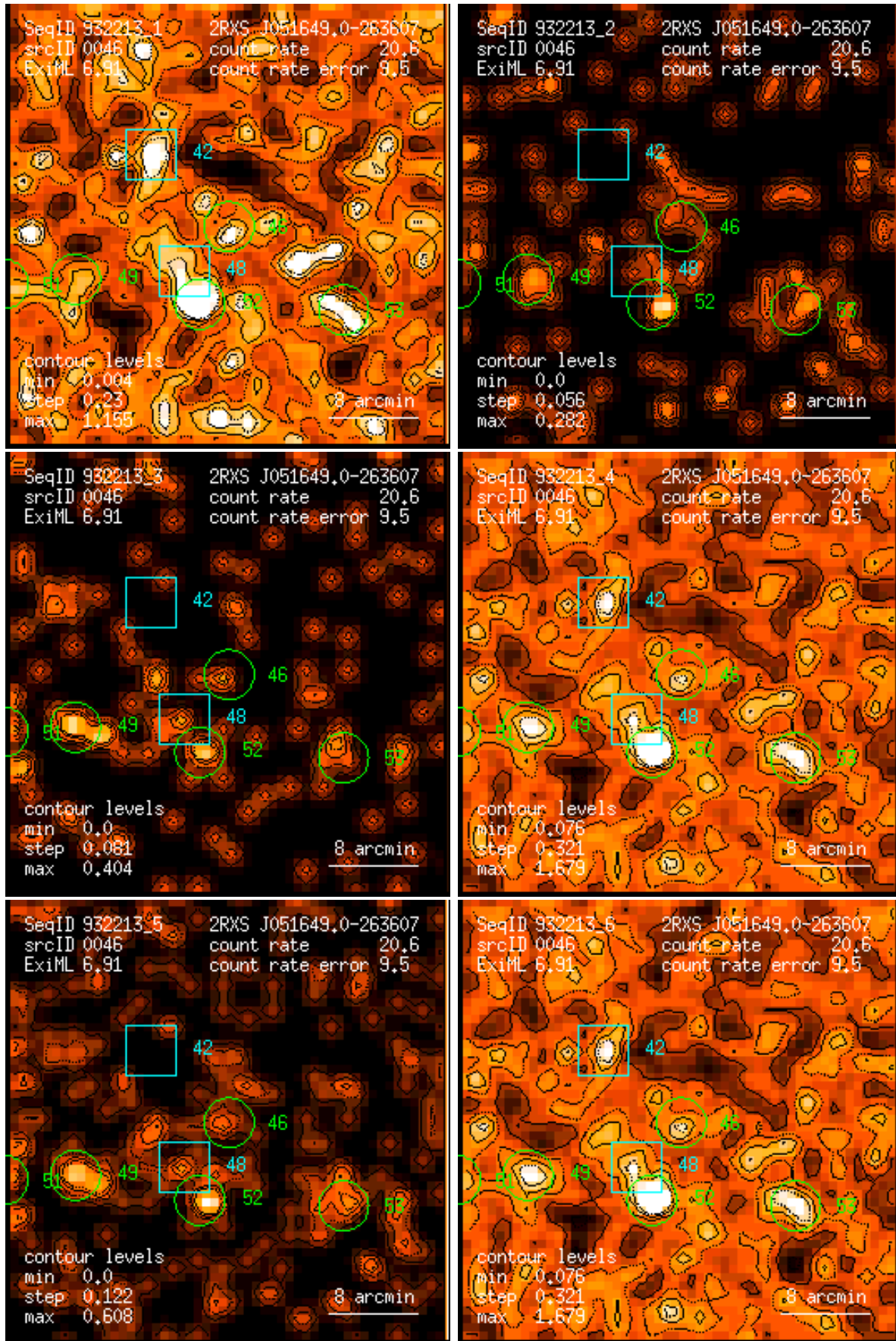
Figure 46: RASS 932213: detection 0046: band rate images, Gaussian filter: (1) PSPC channels 11 – 41, (2) 52 – 90, (3) 91 – 201, (4) 11 – 235, (5) 52 – 201, (6) 11 – 201. Broad band rates in counts/ks. Band rate contour levels in counts/ks/arcmin 2 .
