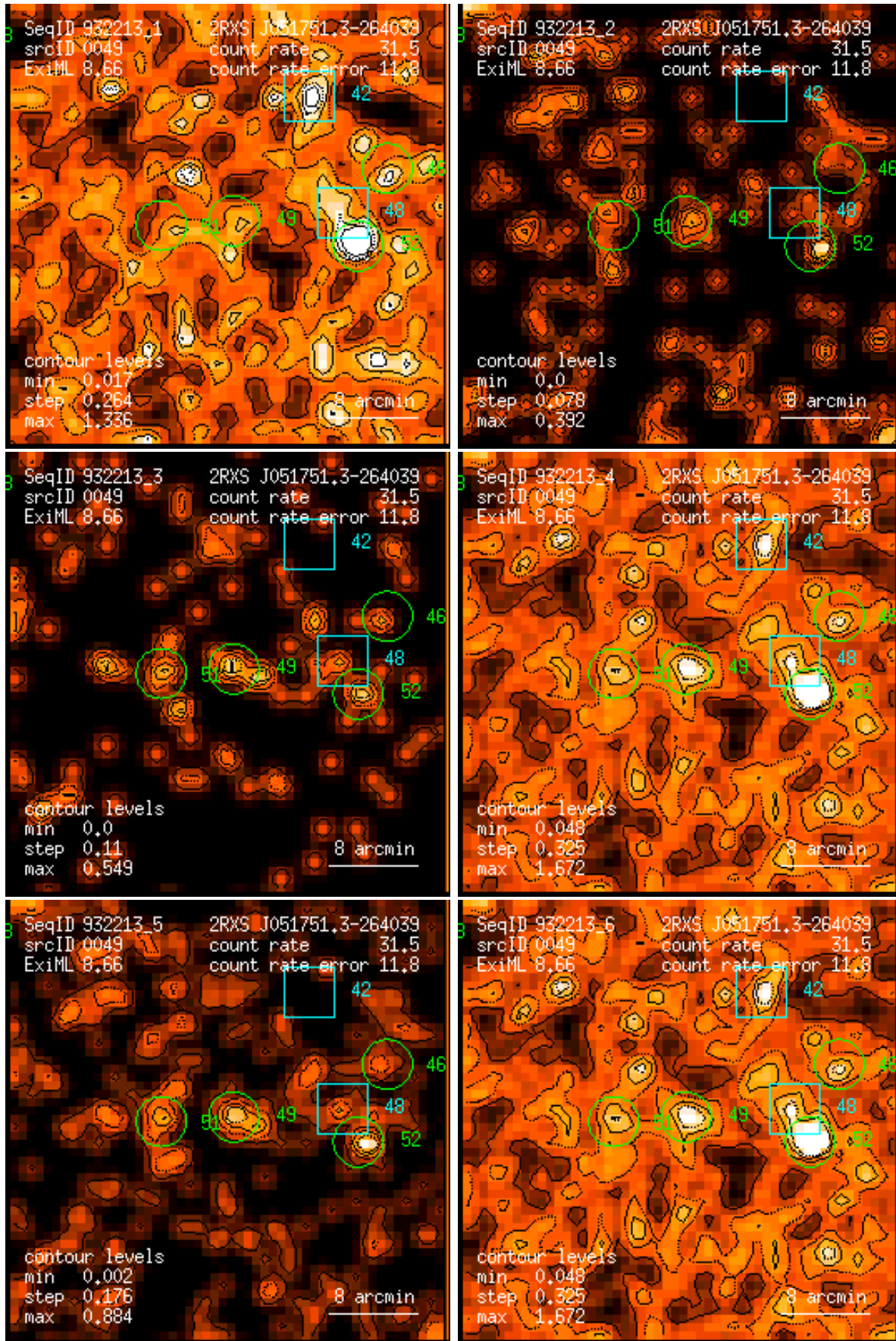
Figure 49: RASS 932213: detection 0049: band rate images, Gaussian filter: (1) PSPC channels 11 – 41, (2) 52 – 90, (3) 91 – 201, (4) 11 – 235, (5) 52 – 201, (6) 11 – 201. Broad band rates in counts/ks. Band rate contour levels in counts/ks/arcmin 2 .
