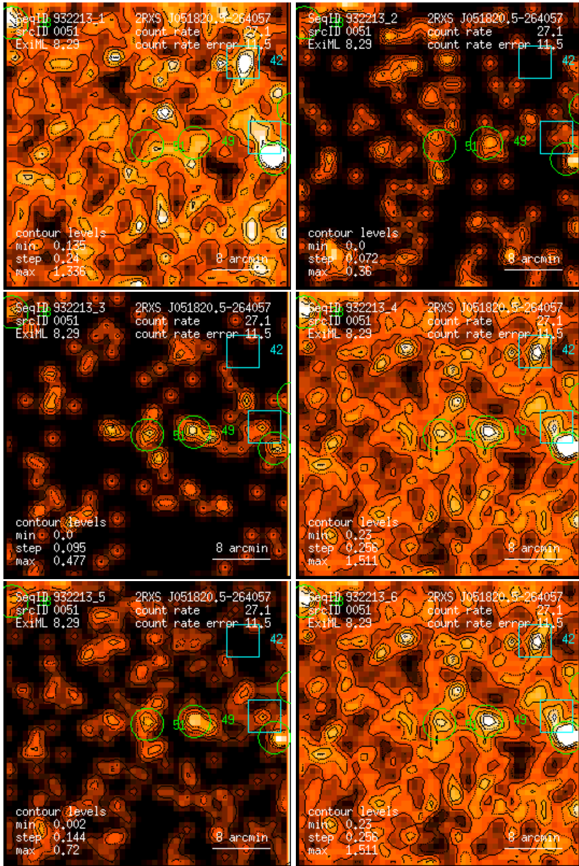
Figure 51: RASS 932213: detection 0051: band rate images, Gaussian filter: (1) PSPC channels 11 – 41, (2) 52 – 90, (3) 91 – 201, (4) 11 – 235, (5) 52 – 201, (6) 11 – 201. Broad band rates in counts/ks. Band rate contour levels in counts/ks/arcmin 2 .
