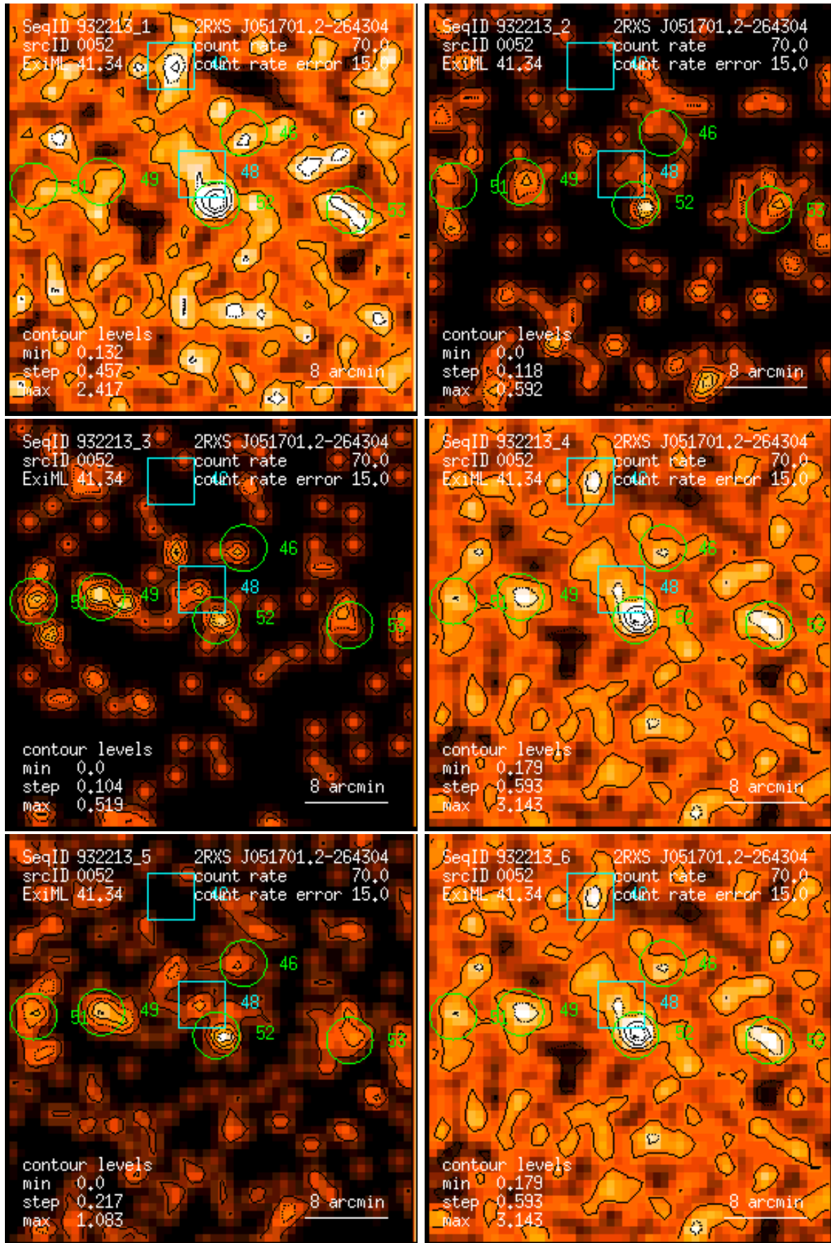
Figure 52: RASS 932213: detection 0052: band rate images, Gaussian filter: (1) PSPC channels 11 – 41, (2) 52 – 90, (3) 91 – 201, (4) 11 – 235, (5) 52 – 201, (6) 11 – 201. Broad band rates in counts/ks. Band rate contour levels in counts/ks/arcmin 2 .
