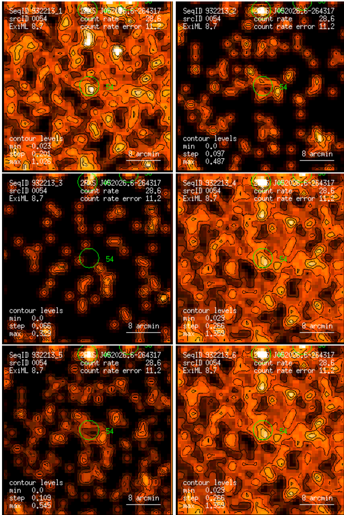
Figure 54: RASS 932213: detection 0054: band rate images, Gaussian filter: (1) PSPC channels 11 – 41, (2) 52 – 90, (3) 91 – 201, (4) 11 – 235, (5) 52 – 201, (6) 11 – 201. Broad band rates in counts/ks. Band rate contour levels in counts/ks/arcmin 2 .
