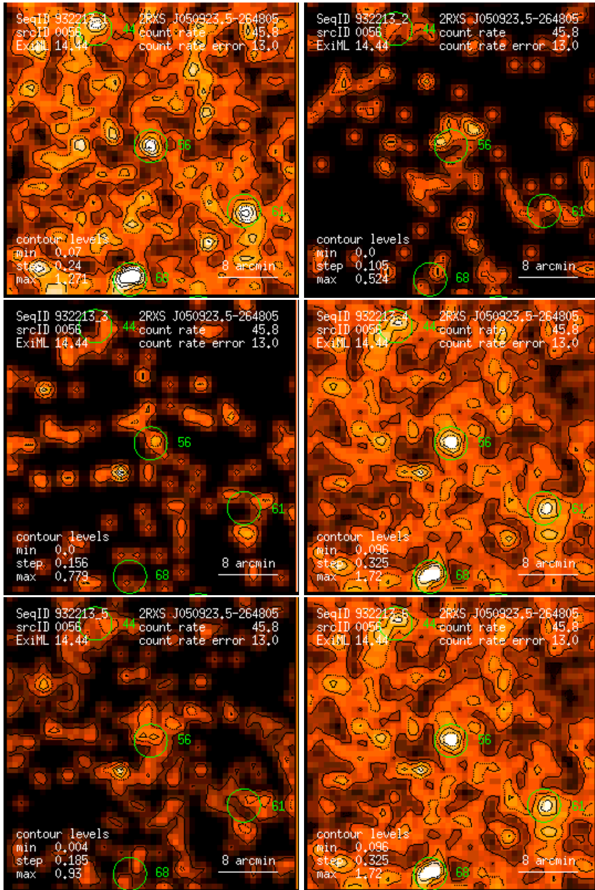
Figure 56: RASS 932213: detection 0056: band rate images, Gaussian filter: (1) PSPC channels 11 – 41, (2) 52 – 90, (3) 91 – 201, (4) 11 – 235, (5) 52 – 201, (6) 11 – 201. Broad band rates in counts/ks. Band rate contour levels in counts/ks/arcmin 2 .
