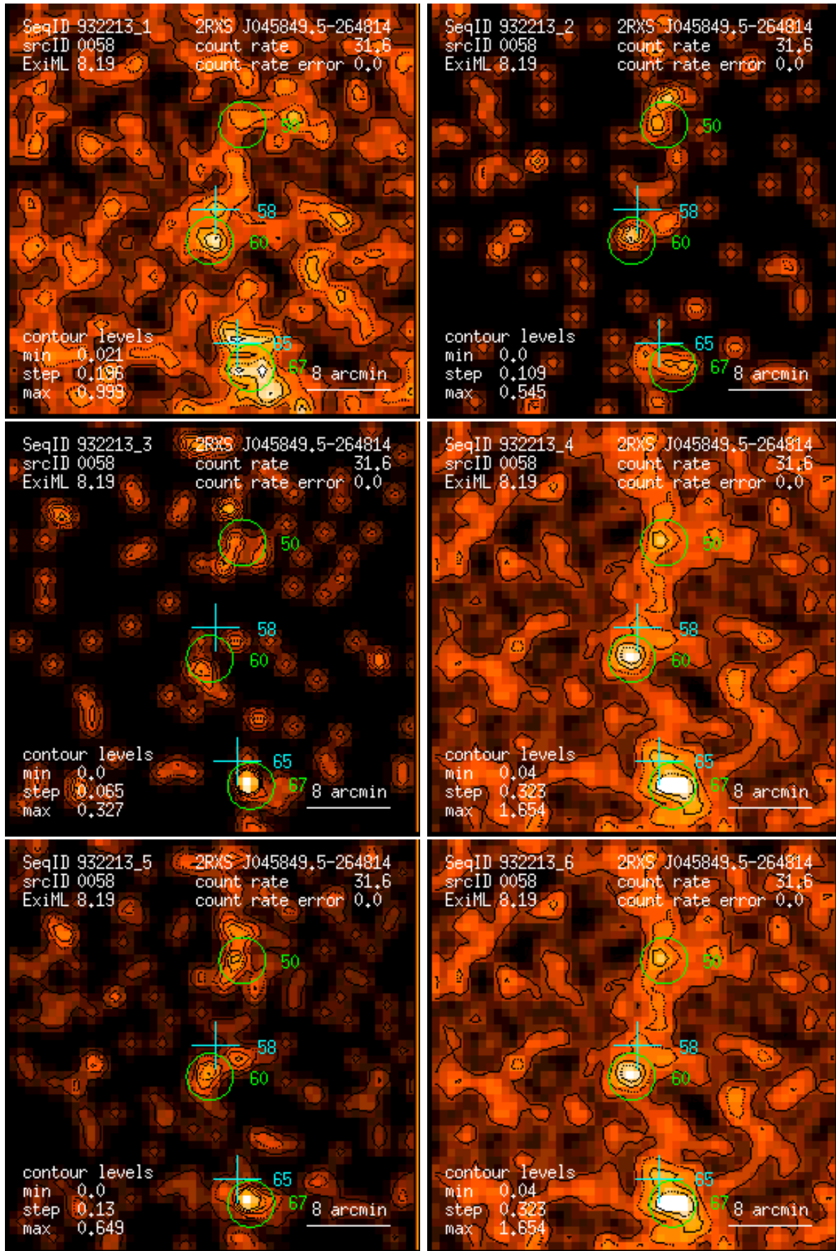
Figure 58: RASS 932213: detection 0058: band rate images, Gaussian filter: (1) PSPC channels 11 – 41, (2) 52 – 90, (3) 91 – 201, (4) 11 – 235, (5) 52 – 201, (6) 11 – 201. Broad band rates in counts/ks. Band rate contour levels in counts/ks/arcmin 2 .
