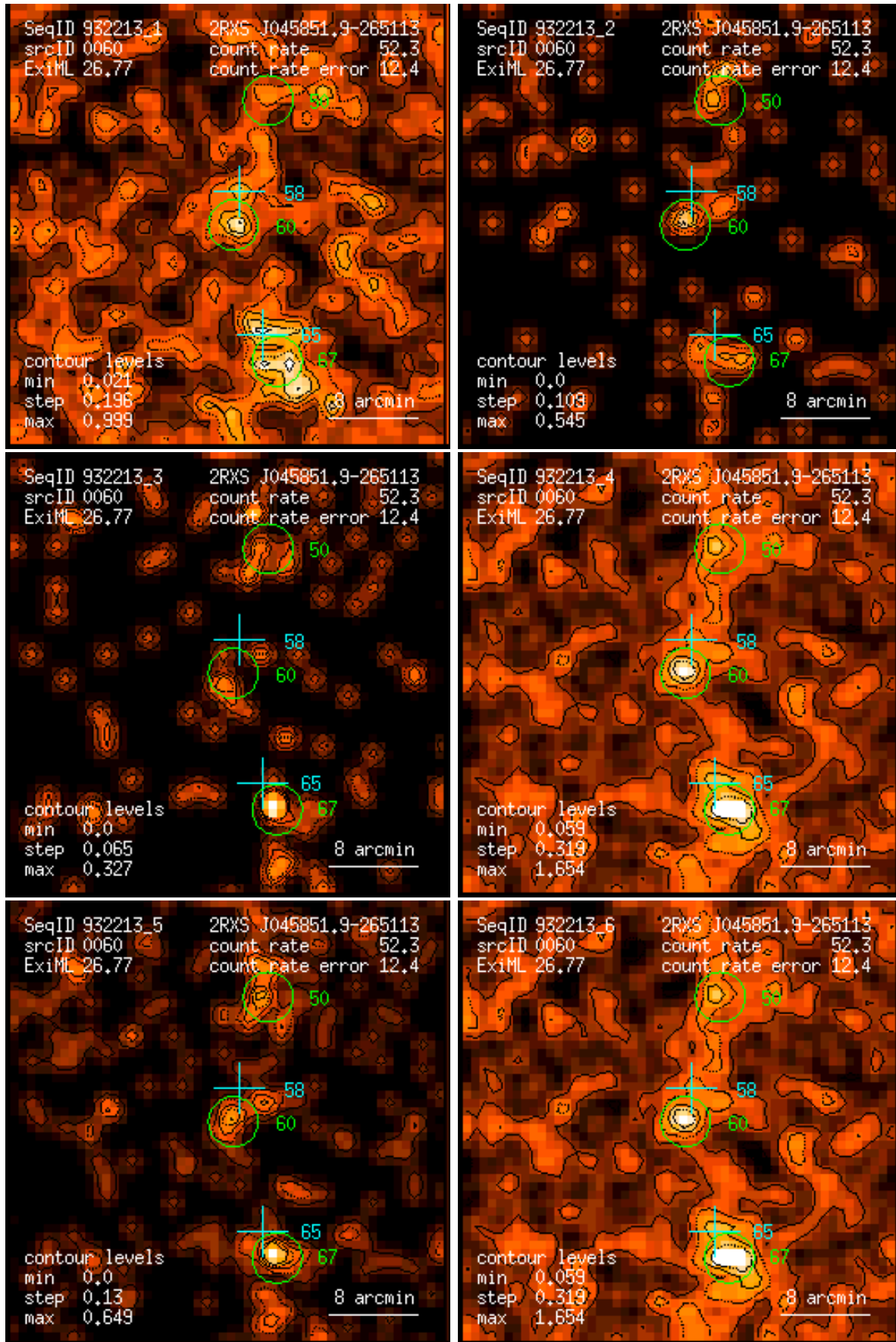
Figure 60: RASS 932213: detection 0060: band rate images, Gaussian filter: (1) PSPC channels 11 – 41, (2) 52 – 90, (3) 91 – 201, (4) 11 – 235, (5) 52 – 201, (6) 11 – 201. Broad band rates in counts/ks. Band rate contour levels in counts/ks/arcmin 2 .
