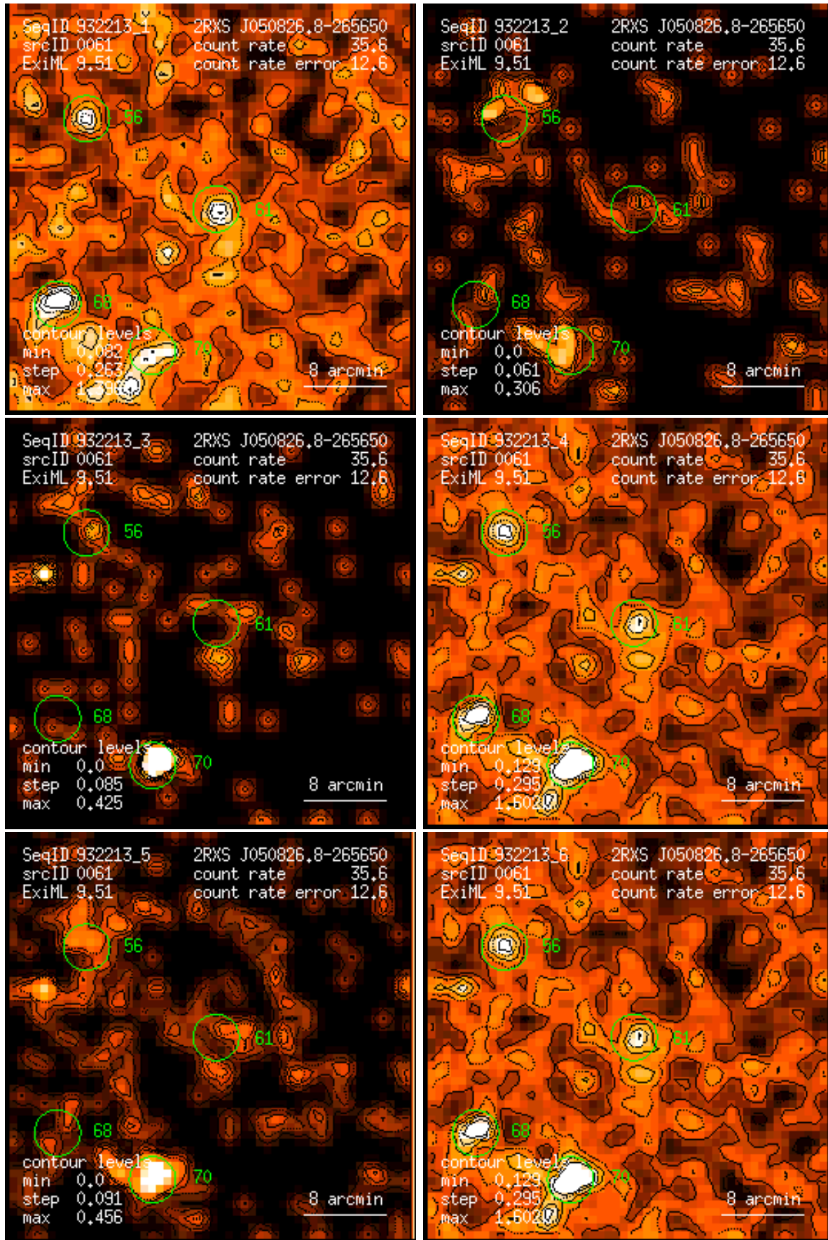
Figure 61: RASS 932213: detection 0061: band rate images, Gaussian filter: (1) PSPC channels 11 – 41, (2) 52 – 90, (3) 91 – 201, (4) 11 – 235, (5) 52 – 201, (6) 11 – 201. Broad band rates in counts/ks. Band rate contour levels in counts/ks/arcmin 2 .
