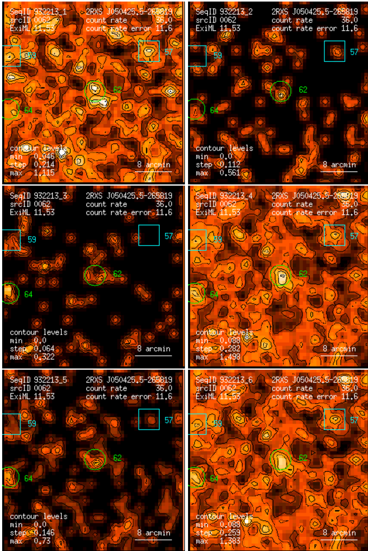
Figure 62: RASS 932213: detection 0062: band rate images, Gaussian filter: (1) PSPC channels 11 – 41, (2) 52 – 90, (3) 91 – 201, (4) 11 – 235, (5) 52 – 201, (6) 11 – 201. Broad band rates in counts/ks. Band rate contour levels in counts/ks/arcmin 2 .
