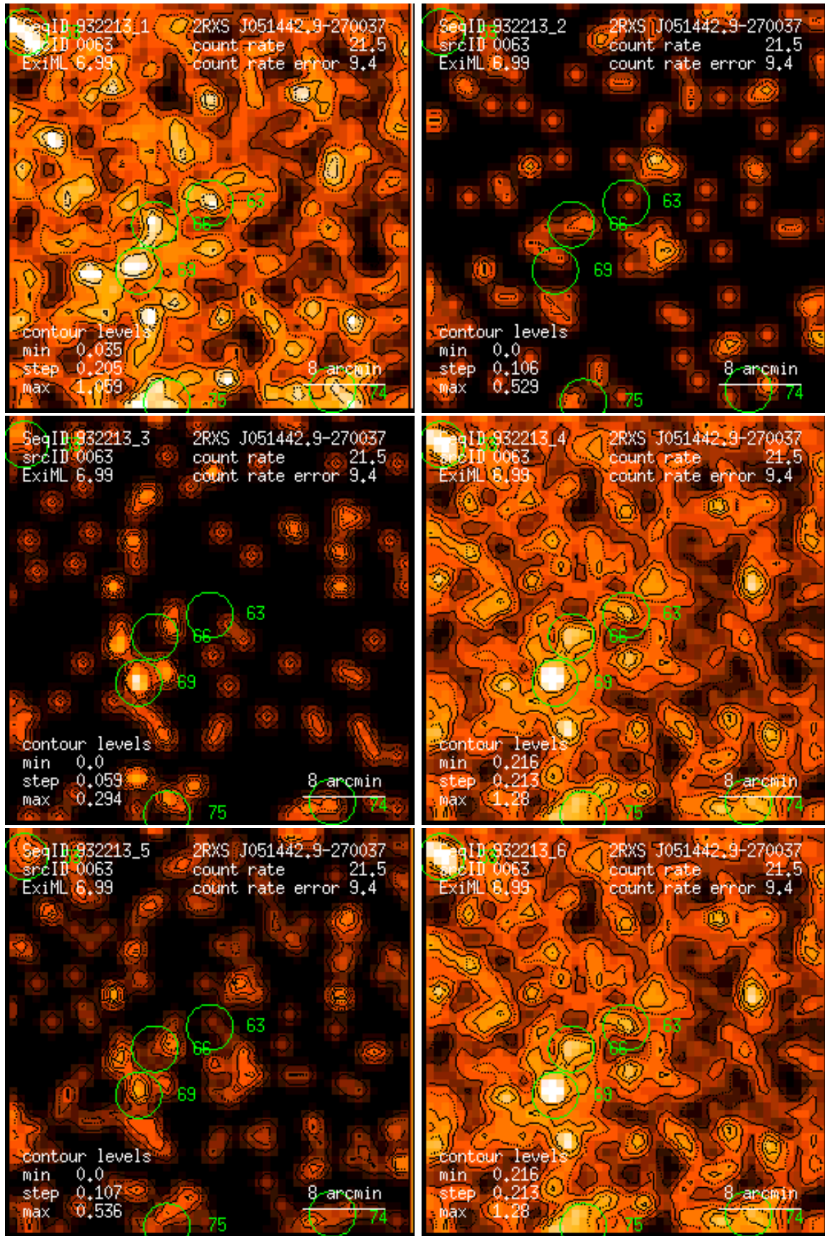
Figure 63: RASS 932213: detection 0063: band rate images, Gaussian filter: (1) PSPC channels 11 – 41, (2) 52 – 90, (3) 91 – 201, (4) 11 – 235, (5) 52 – 201, (6) 11 – 201. Broad band rates in counts/ks. Band rate contour levels in counts/ks/arcmin 2 .
