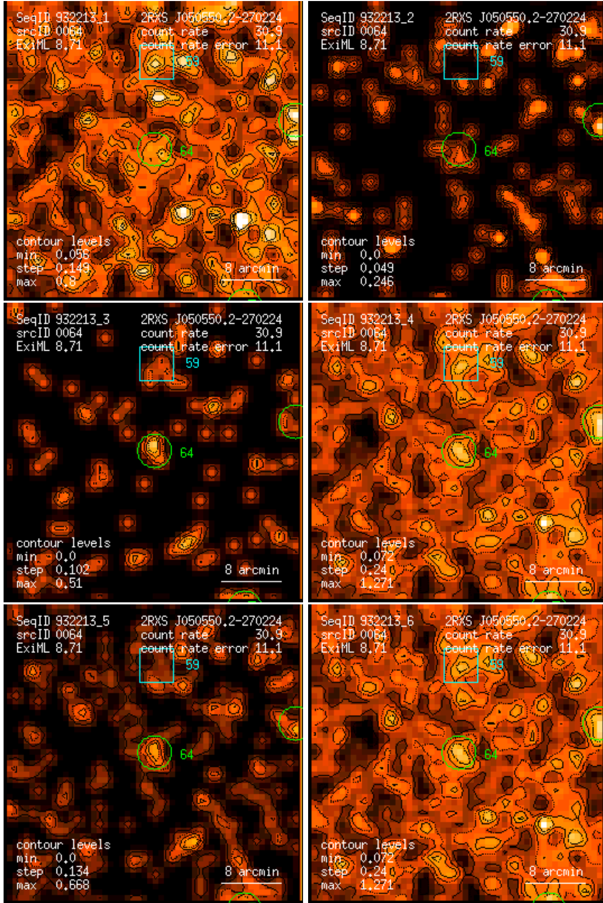
Figure 64: RASS 932213: detection 0064: band rate images, Gaussian filter: (1) PSPC channels 11 – 41, (2) 52 – 90, (3) 91 – 201, (4) 11 – 235, (5) 52 – 201, (6) 11 – 201. Broad band rates in counts/ks. Band rate contour levels in counts/ks/arcmin 2 .
