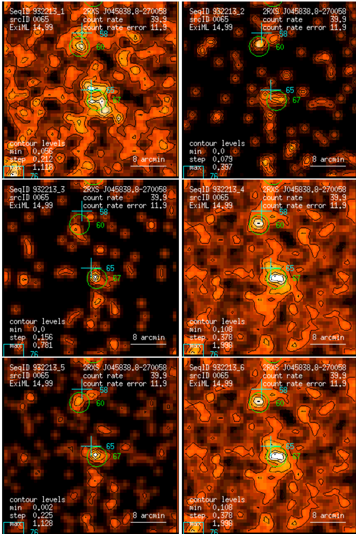
Figure 65: RASS 932213: detection 0065: band rate images, Gaussian filter: (1) PSPC channels 11 – 41, (2) 52 – 90, (3) 91 – 201, (4) 11 – 235, (5) 52 – 201, (6) 11 – 201. Broad band rates in counts/ks. Band rate contour levels in counts/ks/arcmin 2 .
