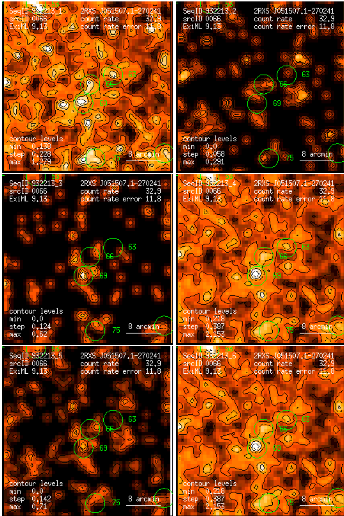
Figure 66: RASS 932213: detection 0066: band rate images, Gaussian filter: (1) PSPC channels 11 – 41, (2) 52 – 90, (3) 91 – 201, (4) 11 – 235, (5) 52 – 201, (6) 11 – 201. Broad band rates in counts/ks. Band rate contour levels in counts/ks/arcmin 2 .
